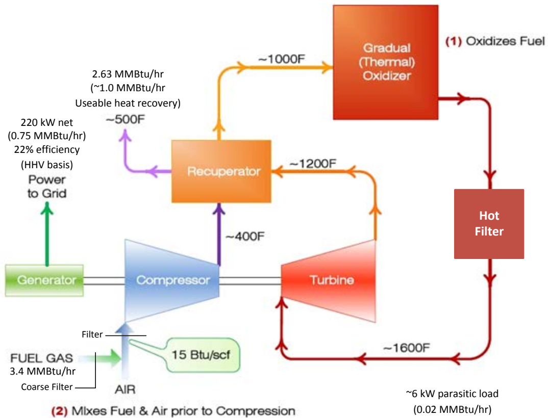
Figure 1. FP250 schematic.
