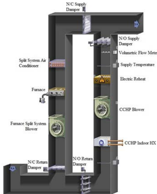
Figure 9. Building integration.
