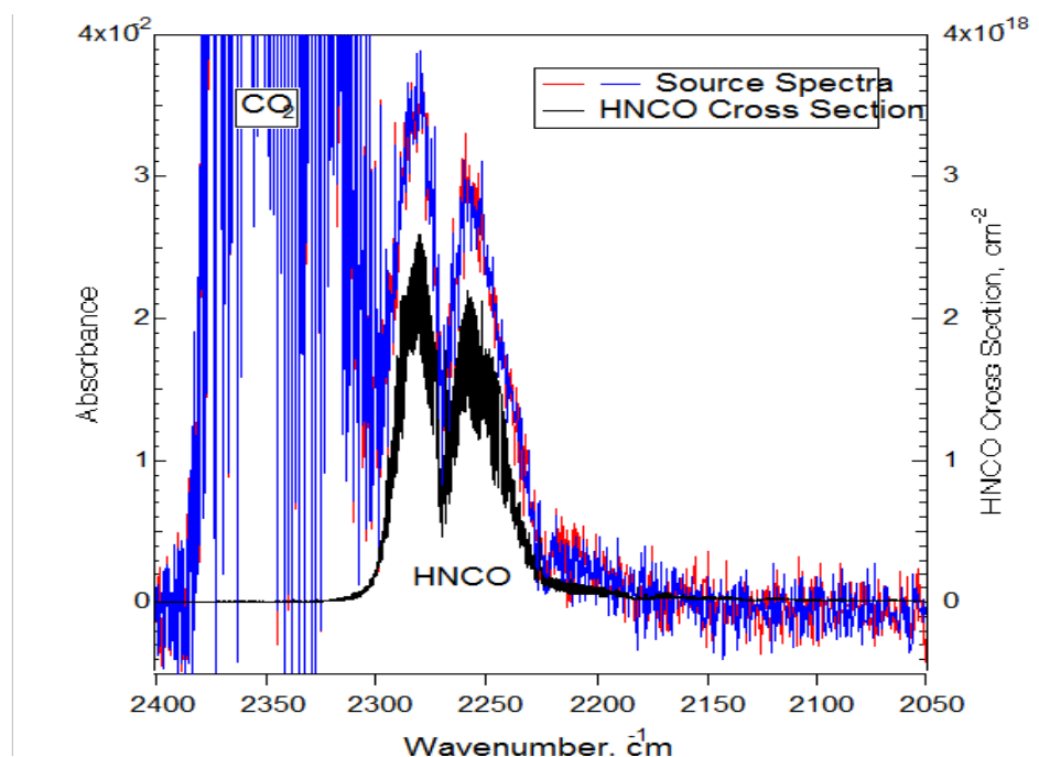
Figure 11.1 Two consecutive infrared spectra of HNCO source output (red, blue) and PNPL reference spectrum (black) as used to quantify the mixing ratio of isocyanic acid during the 2009 Fire Sciences Lab burns.
