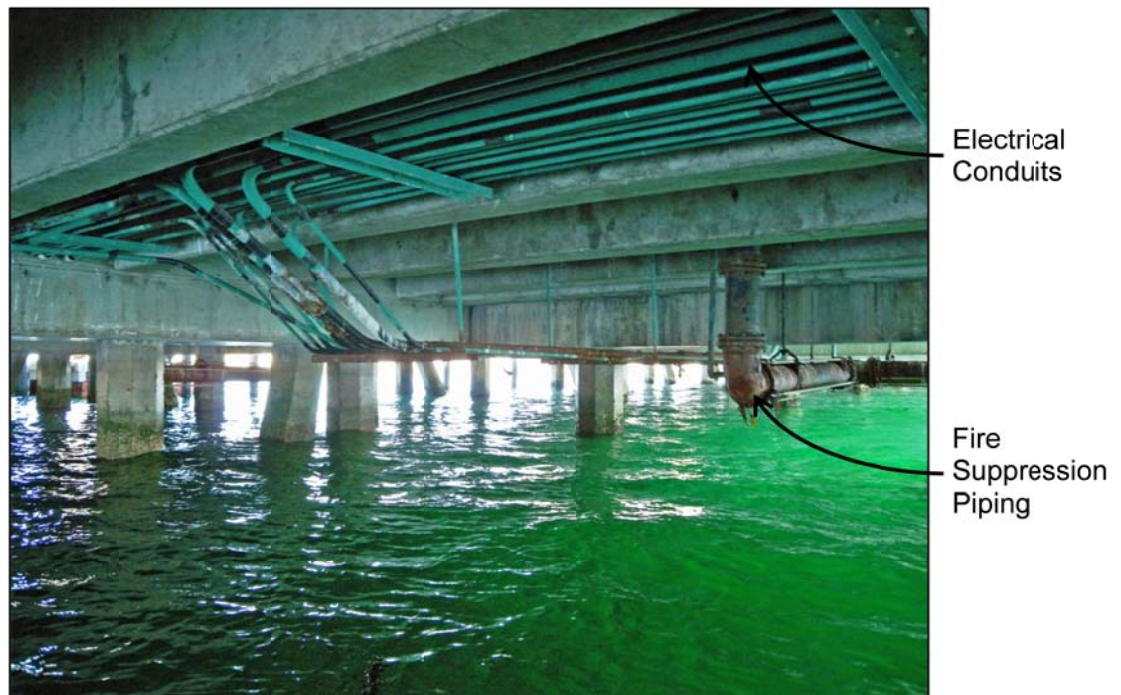
Figure 5-246. The fire suppression piping and electrical conduits at Ammunition Pier Bravo are located below the pier deck.
