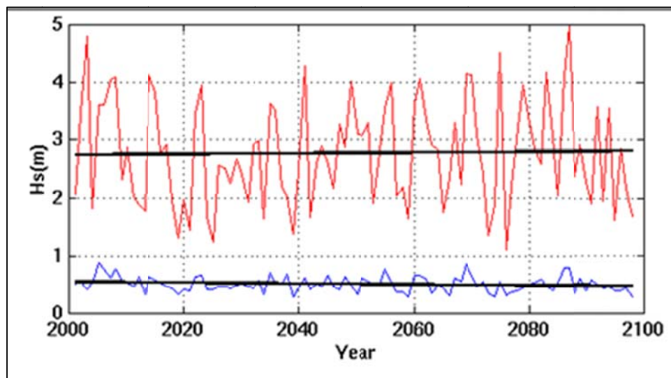
Figure 4-20. Figure 5 22. Annual GCM-derived nearshore wave statistics for MCBCP Range PN1290 including annual significant wave height mean (blue) and maximum (red).
