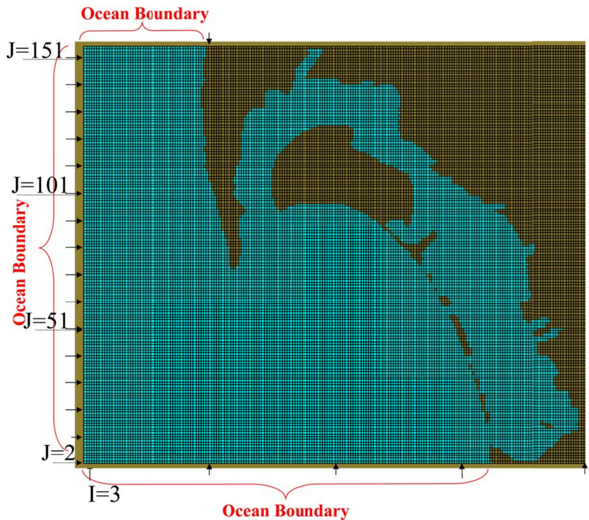
Figure 4-64. Hydrodynamic TRIM model grid for San Diego Bay.
