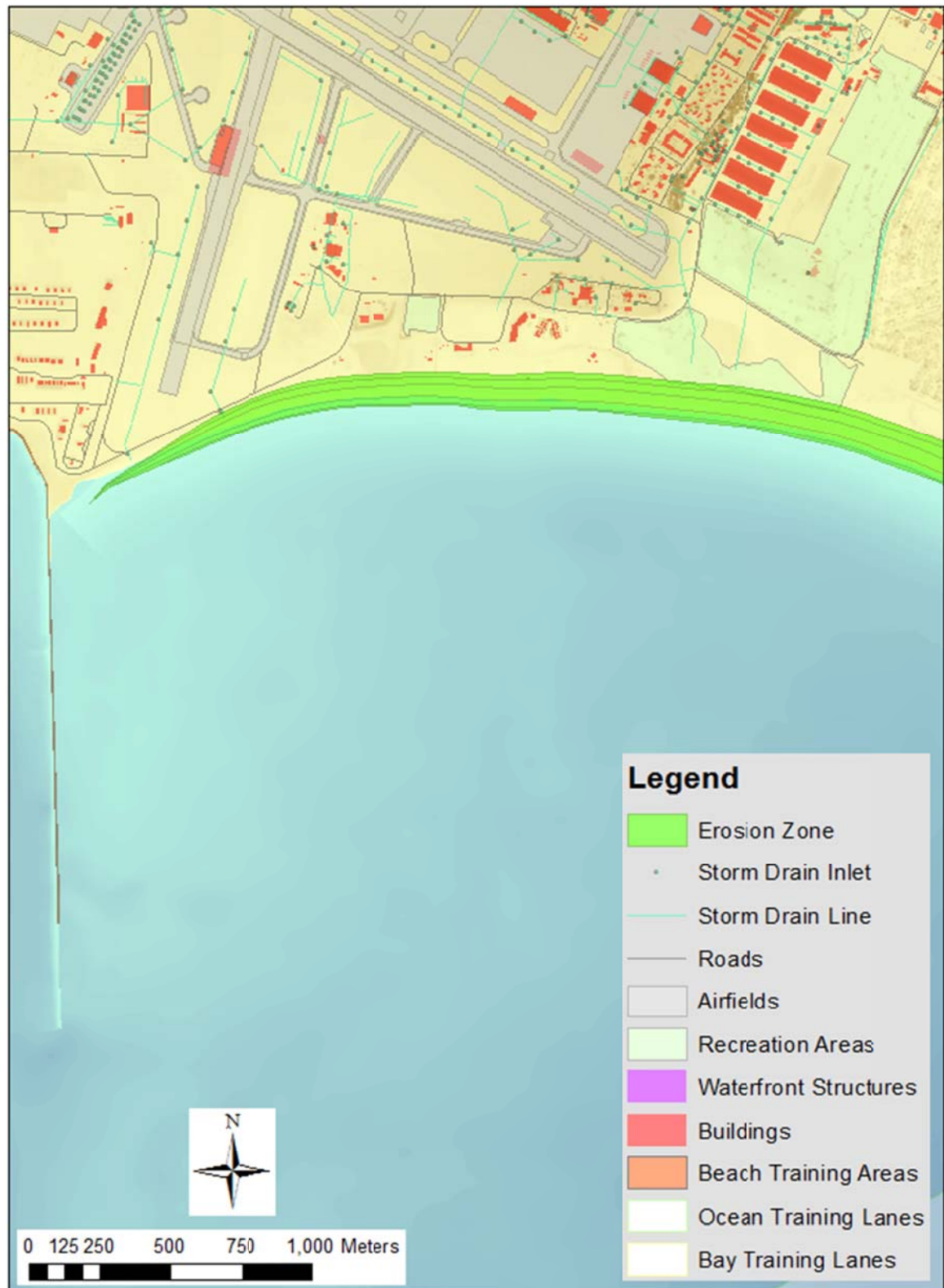
Figure 5-60. Detail view of the erosion footprint for the baseline (SLR=0 m) scenario at North Island. The overall green shaded band spans the 100 year return period wave condition from the YGOR model, and the fine grey lines indicate the shorter return periods ranging from week to decade.
