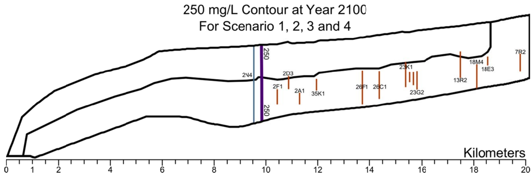
Figure 5-159. Location of the 250 mg/L Chloride contour at year 2100 For the four sea level rise scenarios with the average inland boundary condition. The contour lines are indistinguishable because the distance between the four lines is approximately 35 meters.
