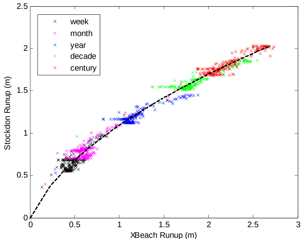
Figure 4-32. Comparison of runup from Stockdon et al. (2006) versus the XBeach results at NBC. The dashed line is a polynomial best fit.
