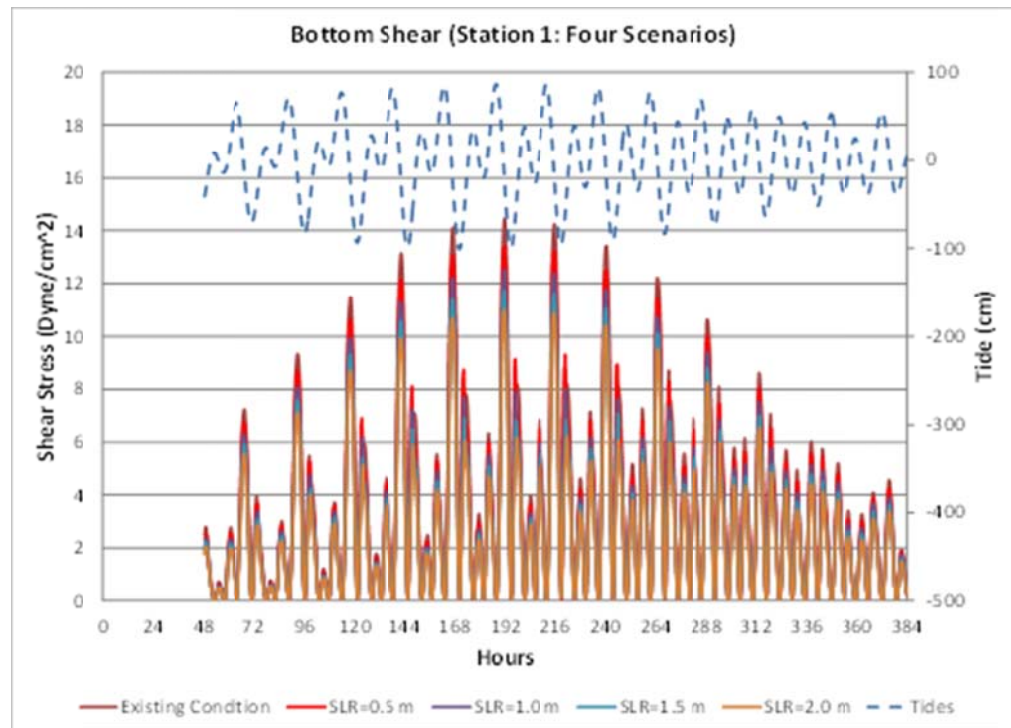
Figure 5-131. Simulated bottom shear stress at Bravo Pier (#1) for the five sea level rise scenarios: baseline, 0.5m, 1m, 1.5m and 2m for a spring-neap tide cycle.
