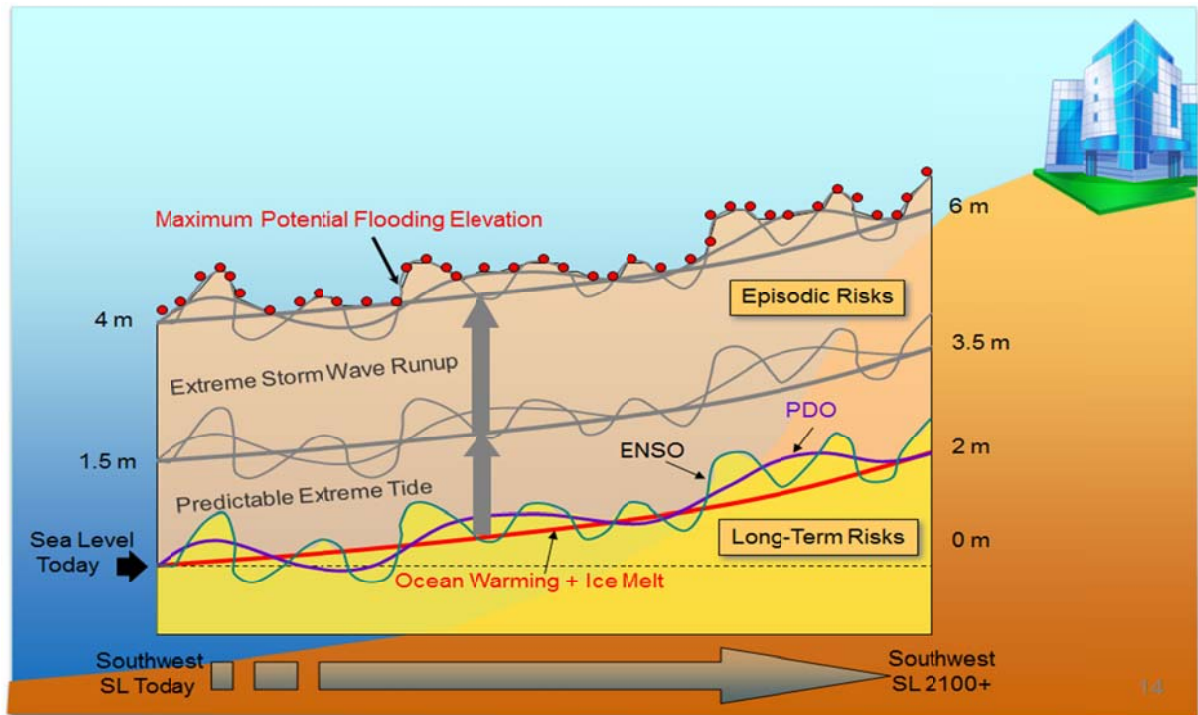
Figure 4-2. Schematic of approximate amplitudes of MSLR, tides, non-tide residual (NTR) variations, and wave-driven runoff during 21st century.
