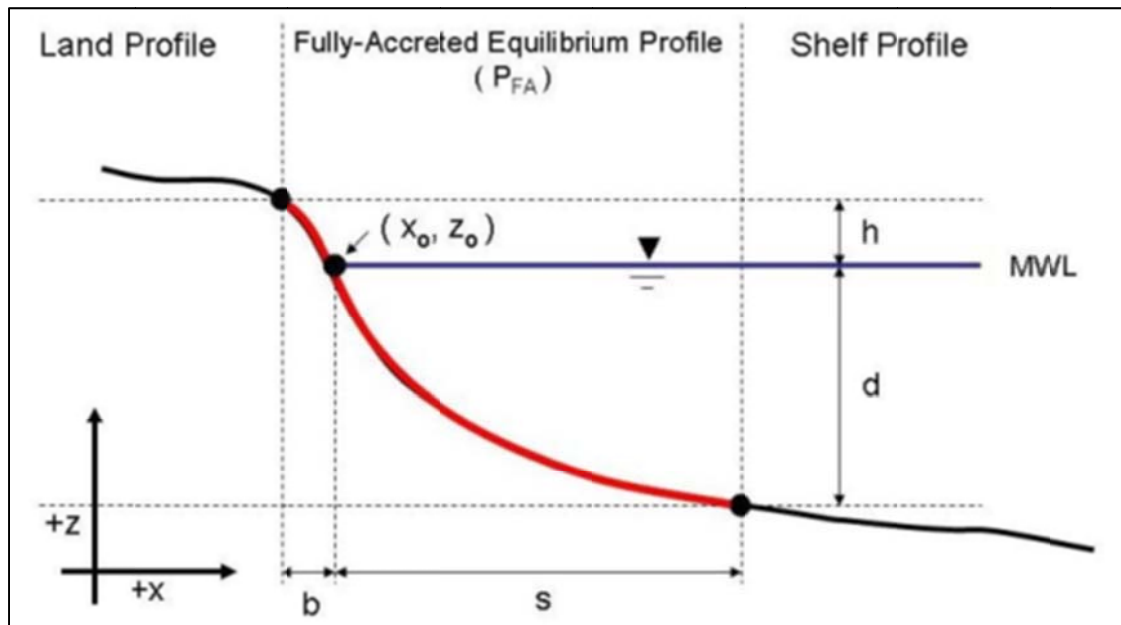
Figure 4-49. Schematic of the fully-accreted summer-dry equilibrium profile.
