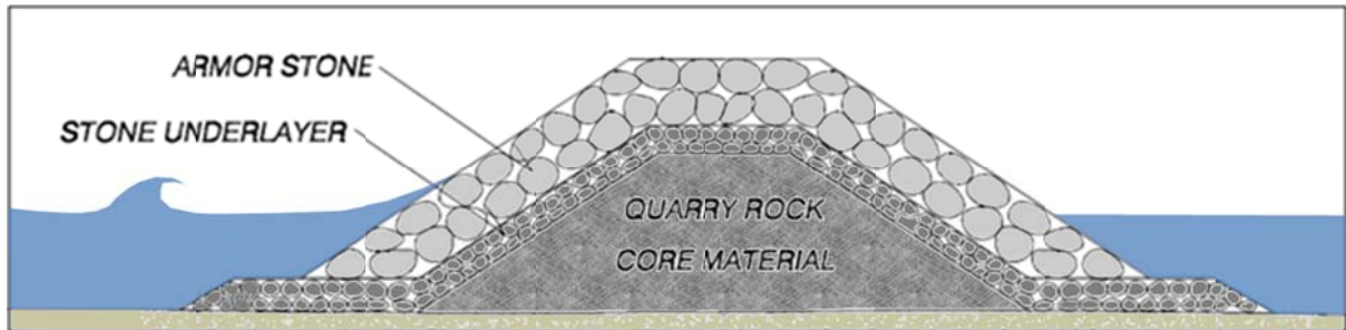
Figure 4-118. Typical rubble-mound jetty section (Adapted from USACE 2006).
