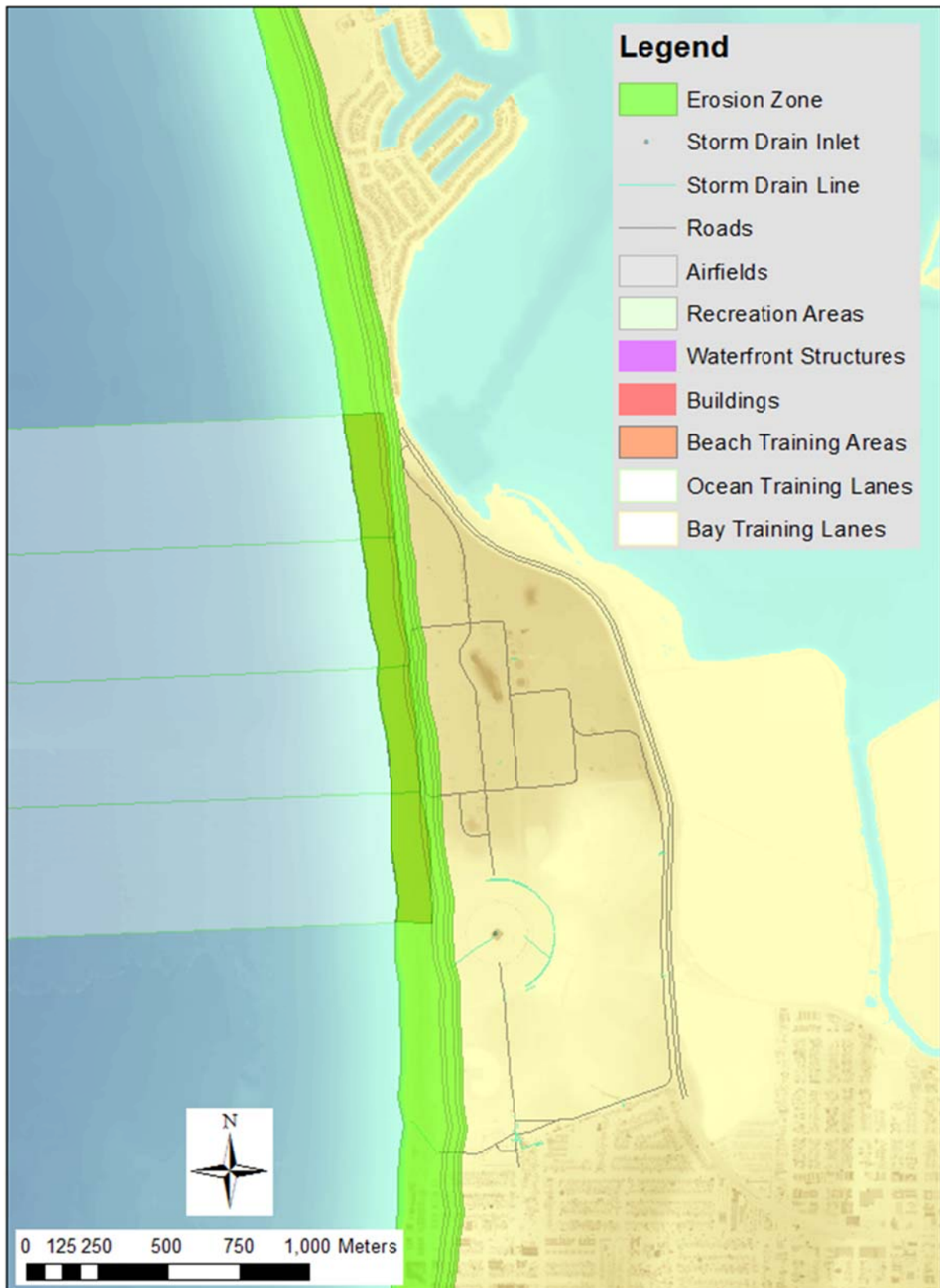
Figure 5-70. Detail view of the erosion footprint for the SLR=2.0 m scenario at SSTC South. The overall green shaded band spans the 100 year return period wave condition from the YGOR model, and the fine grey lines indicate the shorter return periods ranging from week to decade.
