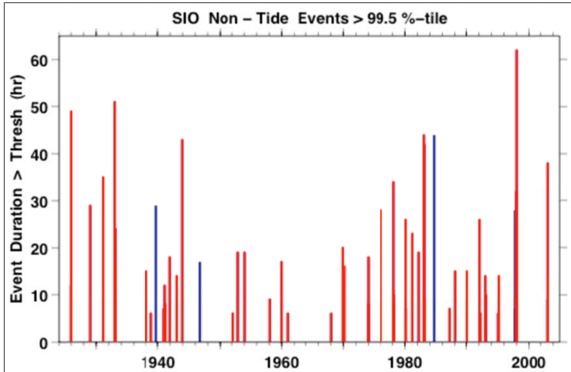
Figure 3-55. Duration (hours) of the 63 extreme NTR events that exceeded the 99.5th percentile during the full year (red) and non-winter (April-September, blue).
