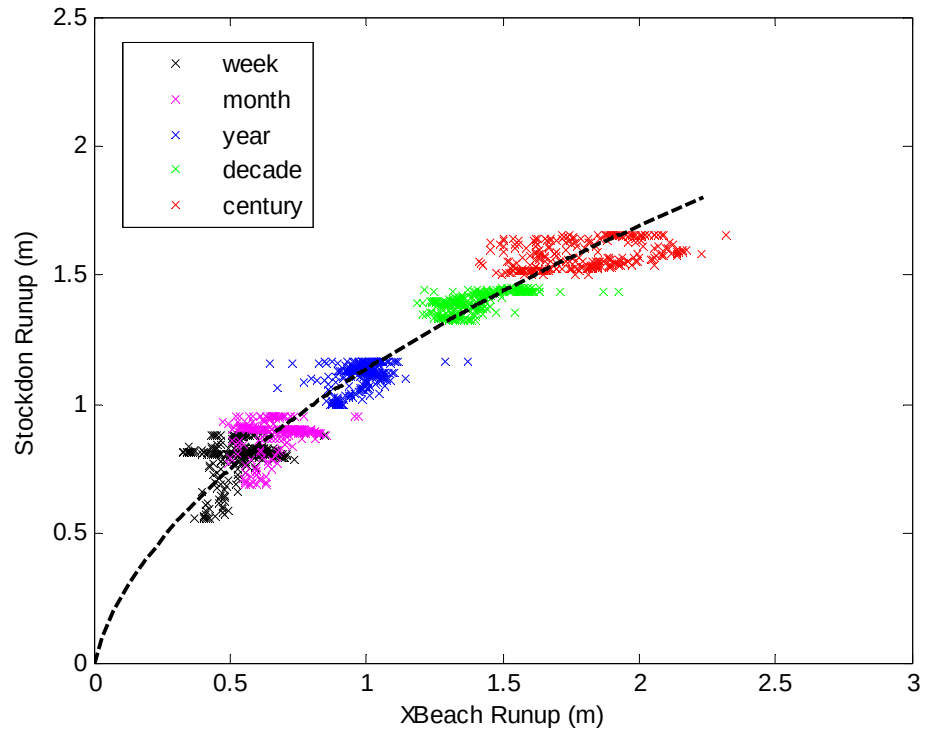
Figure 4-33. Comparison of runup from Stockdon et al. (2006) versus the XBeach results at MCBCP. The dashed line is a polynomial best fit.
