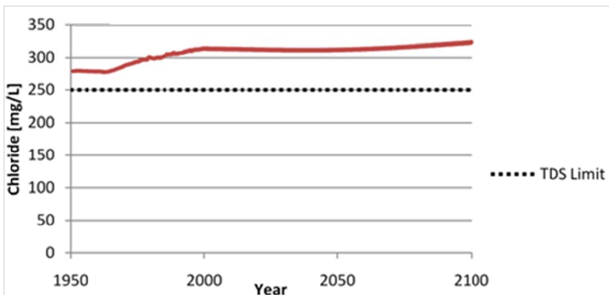
Figure 5-146. 11S005W02N004S (2N4) simulated Breakthrough curve from 1950 to 2100 with no sea level rise.
