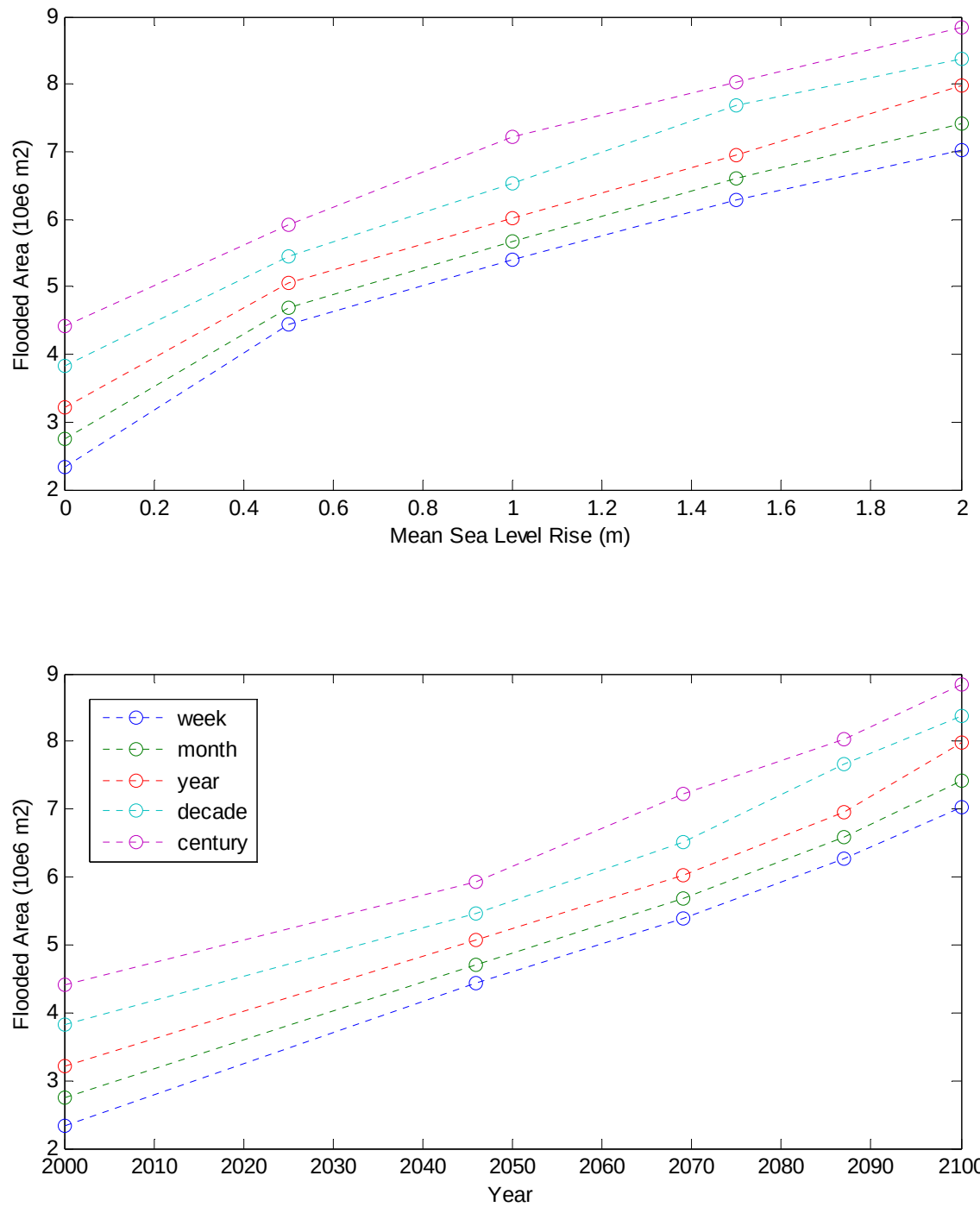
Figure 5-100. Estimated area vulnerable to inundation and flooding (cropped to NAVD88=0m) for the 25 scenarios at MCBCP as a function of mean sea level rise (above) and time (below).
