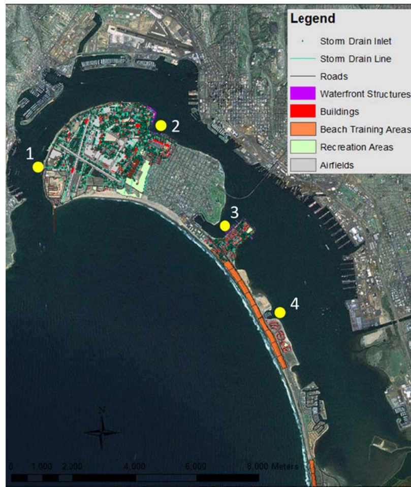
Figure 5-125. Station locations for the model simulations shown in Figure 5-126 – Figure 5-135.
