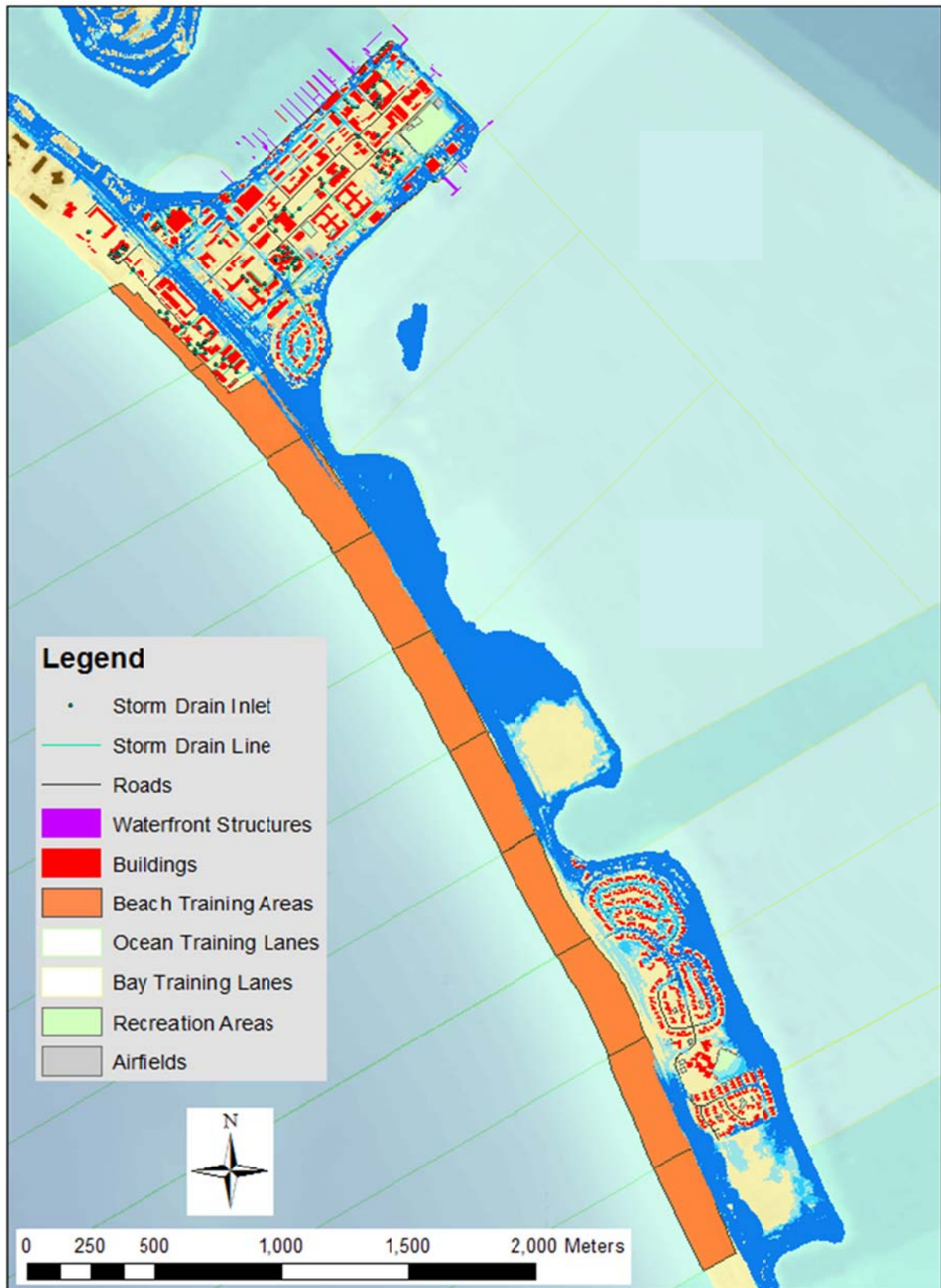
Figure 5-123. Detailed view of inundation and flooding for the 2.0 m SLR bay-exposure scenario at NAB/SSTC North. The blue shaded zones represent week (dark blue), year (medium blue) and century (light blue) return periods.
