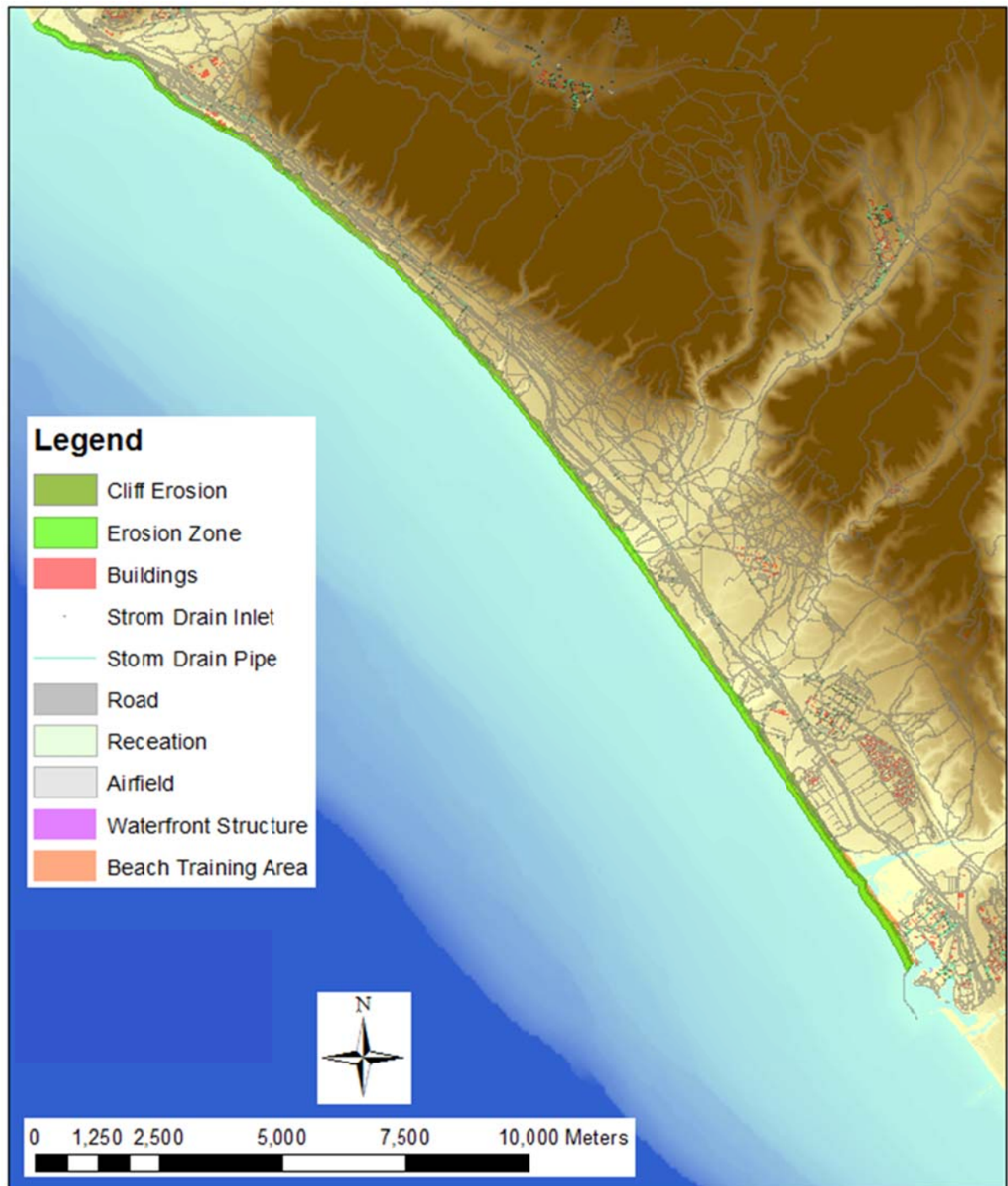
Figure 5-79. Erosion footprint for the SLR=1.0 m scenario at MCBP. The overall light green shaded band spans the 100 year return period wave condition from the YGOR model, and the fine grey lines indicate the shorter return periods ranging from week to decade. The dark green shaded band indicates the extent of cliff erosion.
