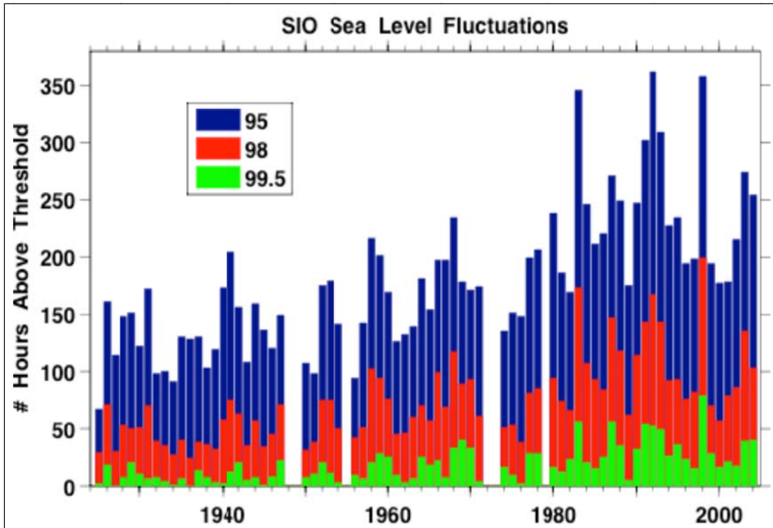
Figure 3-53. Number of winter (November-March) hours that water levels exceed given percentile thresholds (see text).
