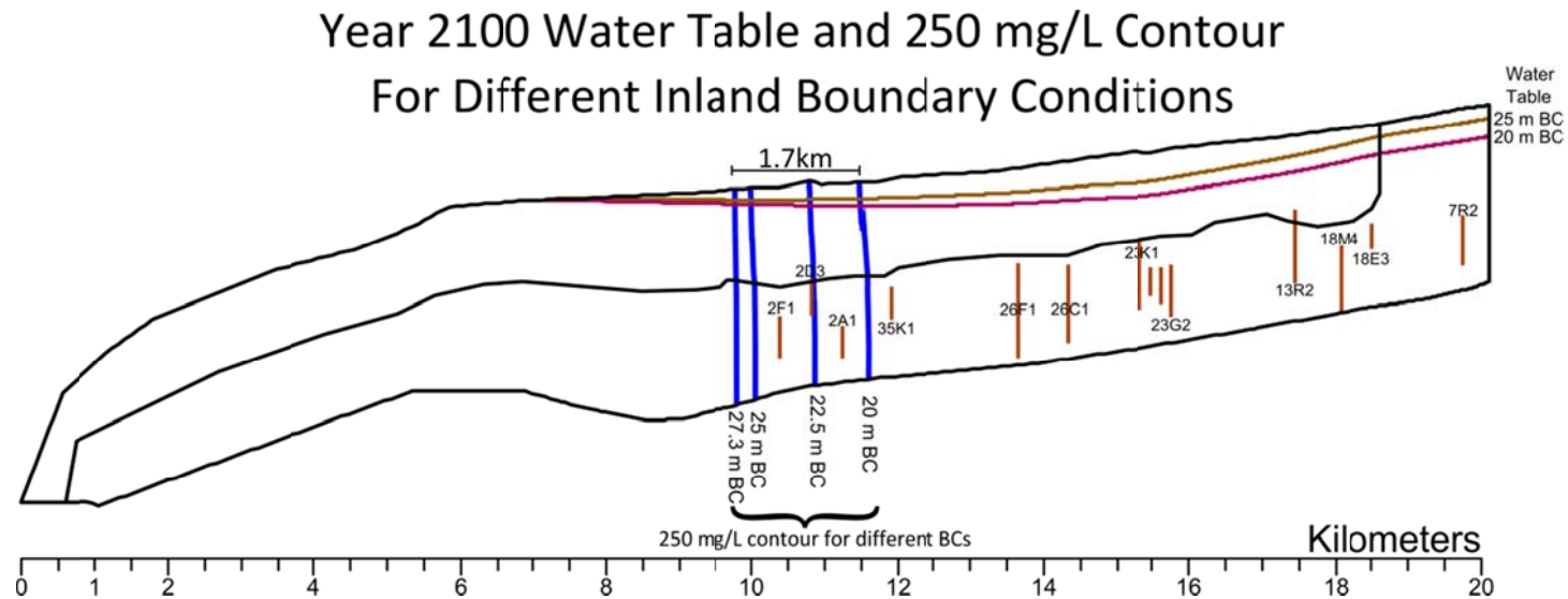
Figure 5-161. Location of the 250 mg/L Chloride contour line and water table at year 2100 for different 2000 to 2100 constant boundary conditions (BC) for Scenario 4. Note that this image has been scaled 1:50 in the vertical direction and that the 27.3 m BC is the average water level of 7J1.
