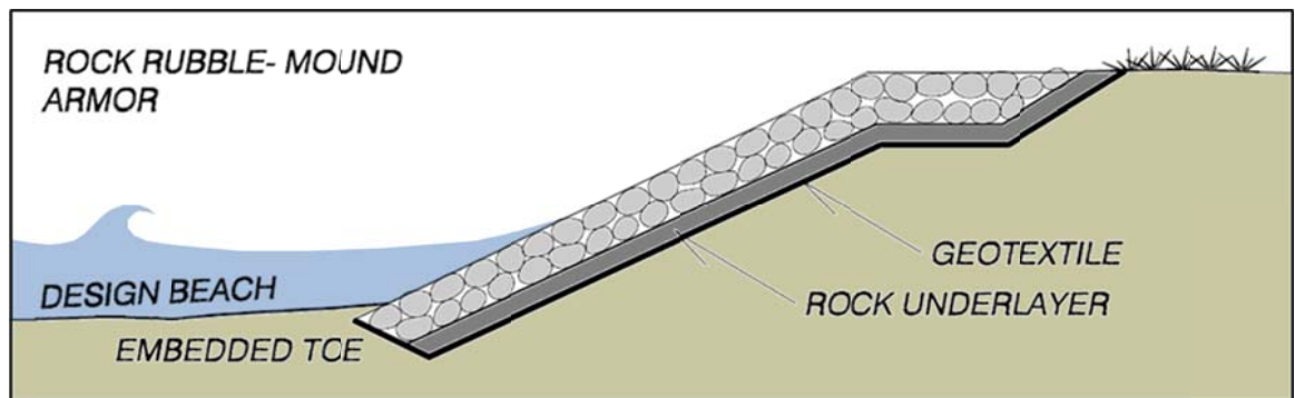
Figure 4-116. Typical rubble-mound revetment section (Adapted from USACE 2006).
