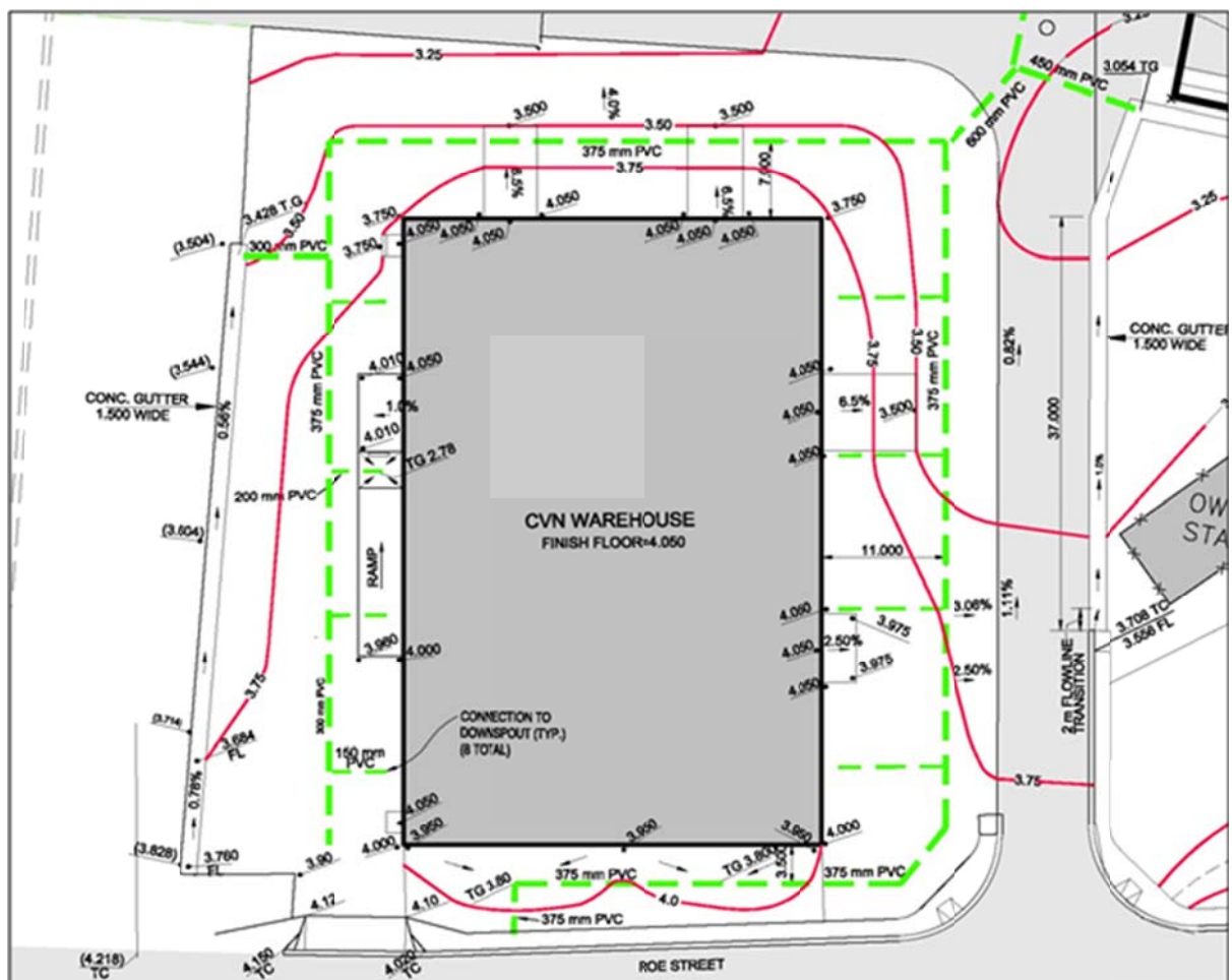
Figure 5-230. An excerpt from the Record Drawings grading plan for the construction of the Berth Juliet wharf, buildings and other improvements. The red lines indicate elevation contours in meters relative to MLLW. The green dashed lines indicate a below grade storm water drainage system.
