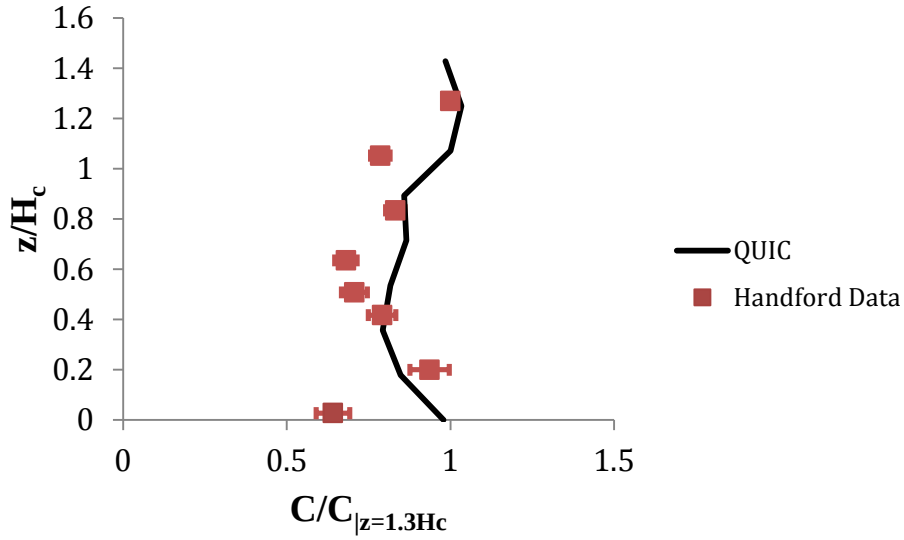
Figure 34: The variation of concentration with height within the canopy at Hanford, WA. The field data indicates that concentration, C increases with height in an irregular manner that is generally followed by the QUIC simulation except near the ground. These data were taken 32 m downwind of the road. Error bars indicate 95% confidence intervals.
