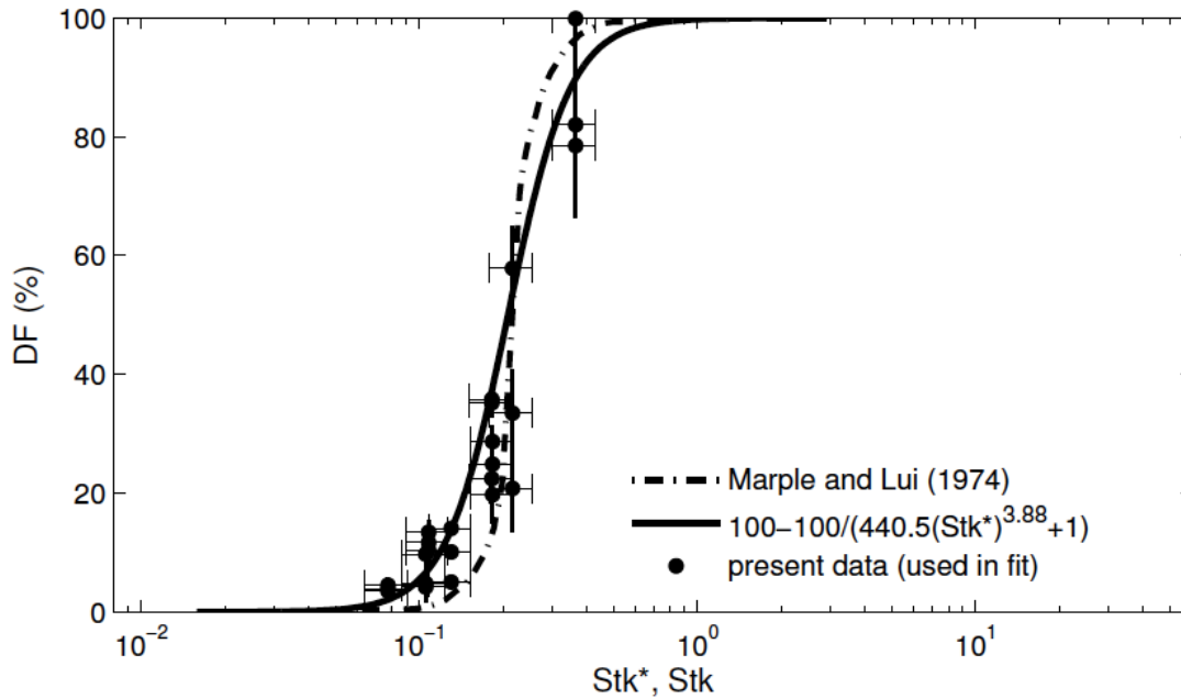
Figure 28: Deposition fraction, DF, as a function of Stk^* showing the collapse of the artificial substrate data.
