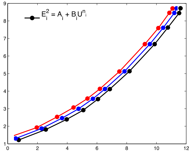
Figure 6: Hot-wire probe velocity ( U ) – voltage ( E ) calibration curve. Calibration was performed both before (subscript i) and after (subscript f) data collection in the wind tunnel. The average curve (subscript ave) was used to process the data. A , B and n represent best-fit coefficients.
