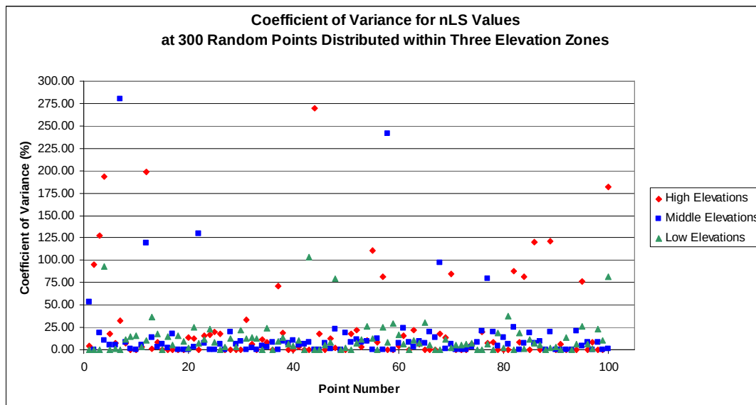
Figure 34. Coefficient of variation for accumulated nLS+ values at 300 random locations, across three elevation zones, at the Kahuku Training Area, Schofield Barracks, Oahu.
