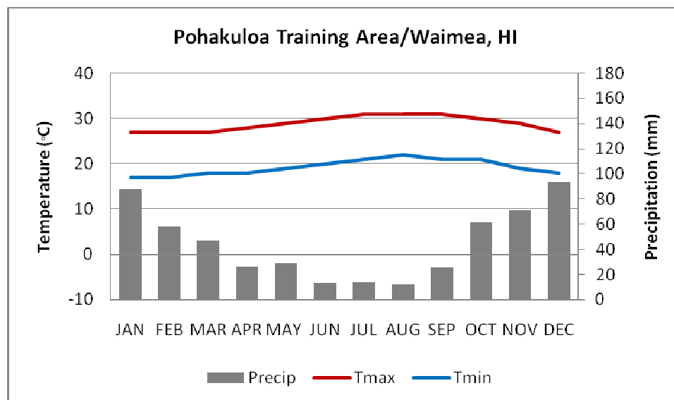
Figure 26. Climograph for Pohakuloa Training Area, Hawaii (Source: http://www.weather.com ).
