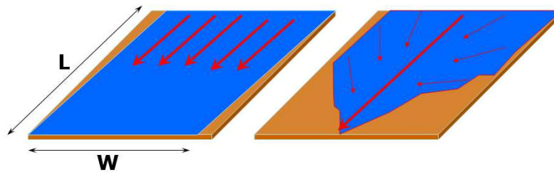
Figure 1. Schematic illustrating the difference between sheet and concentrated flows.
