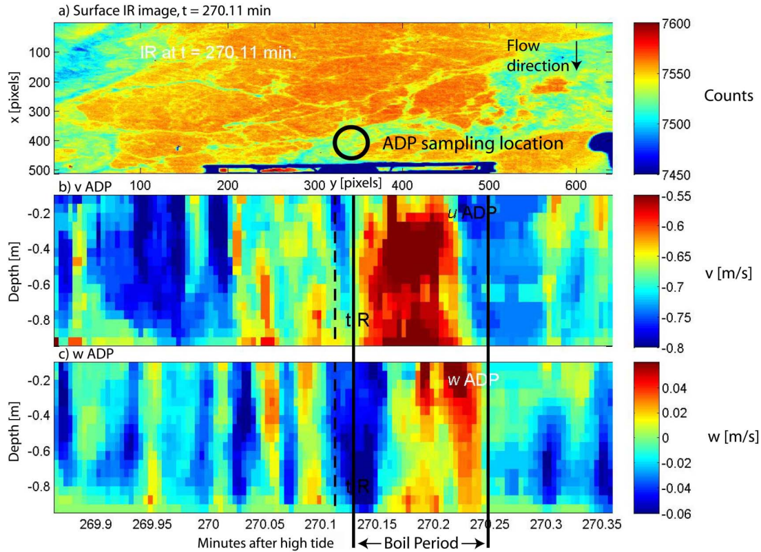
Figure C2: a) Uncalibrated IR image showing a passing boil (warm colors) on the water surface. The typical temperature range is less than 0.7^{\circ}\text{K} . Profiles of b) streamwise horizontal and c) vertical velocity measured with the ADP at the location indicated in a). The dashed line corresponds to the time of the IR image.
