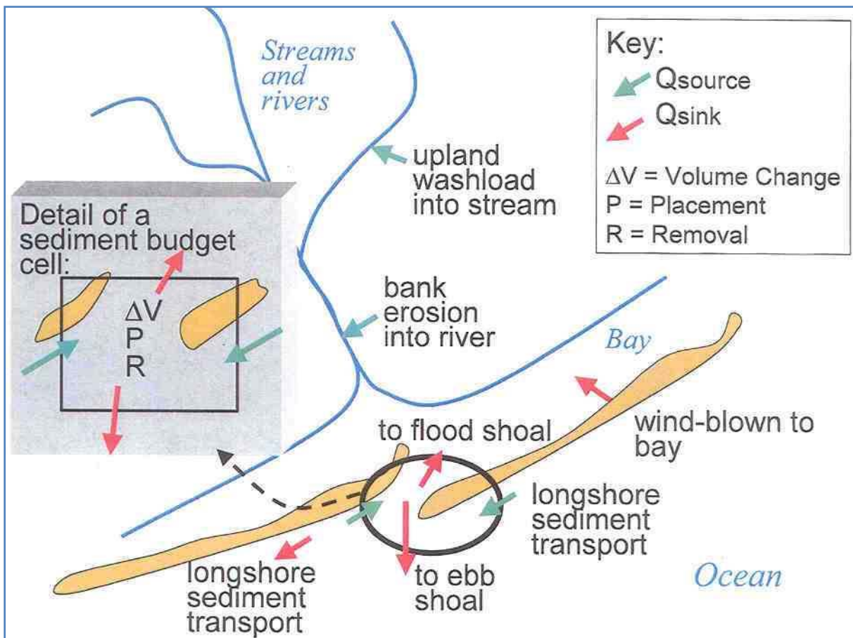
Figure 1. Sediment budget parameters that may enter Equation 1.
