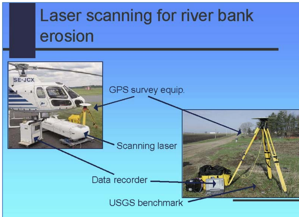
Figure 5. LIDAR system.
