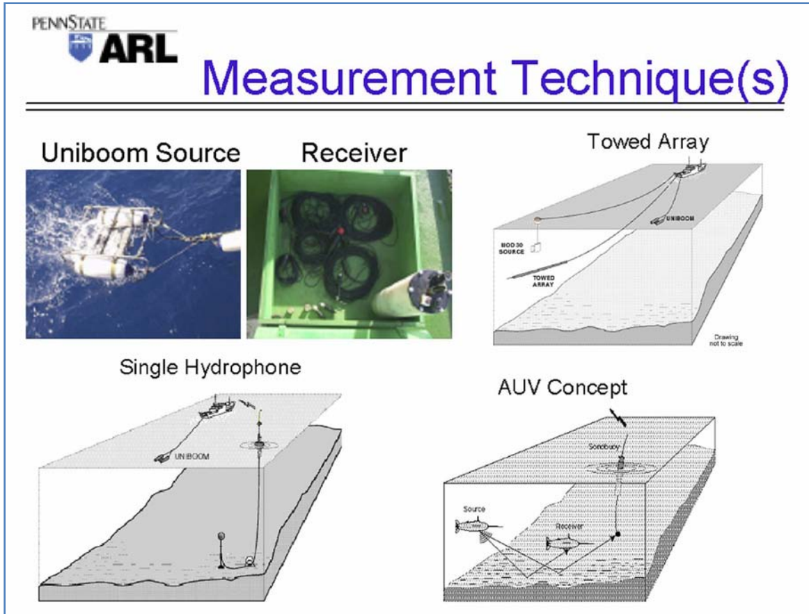
Figure 3. Pennsylvania State University, Applied Research Laboratory (ARL), deployment/measurement scheme. (Note: AUV = Autonomous Unmanned Vehicle).
