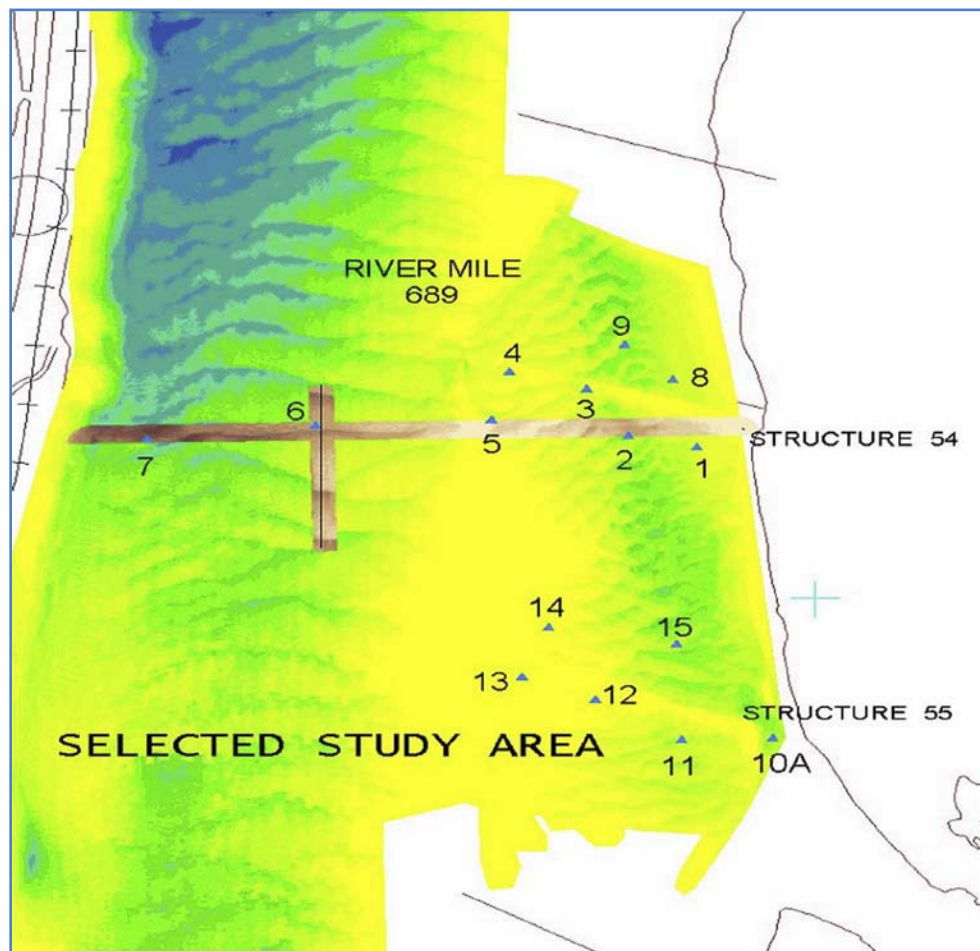
Figure 6. Small section of bathymetric data taken at Pool 8. The brown areas represent special timed lateral and longitudinal swaths.
