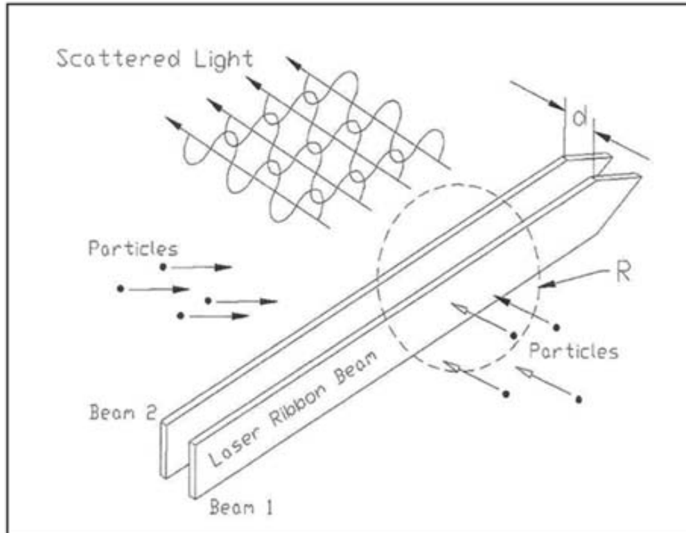
Figure 9. Simplified diagram of the two-beam technique.
