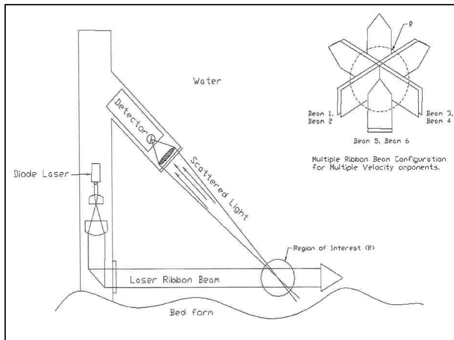
Figure 10. Laser and detector configuration, and multiple ribbon beam configuration.
