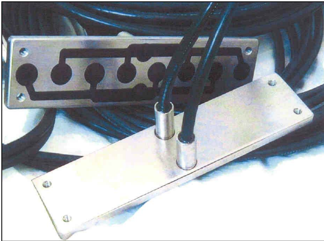
Figure 7. Seatek stainless steel sensor rack.
