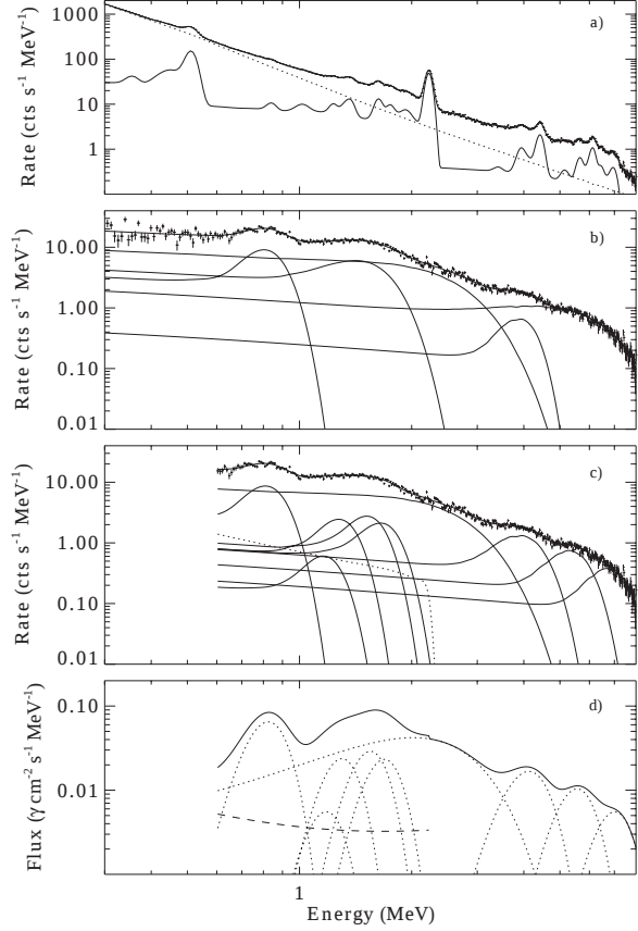
Figure 1: a) Summed spectrum from 19 flares observed by SMM; b) spectrum with narrow lines and bremsstrahlung removed fit by 5 broad Gaussians; c) same as 1b) but fit by several components from 0.6 to 8.0 MeV (see text); d) derived incident photon spectrum.
