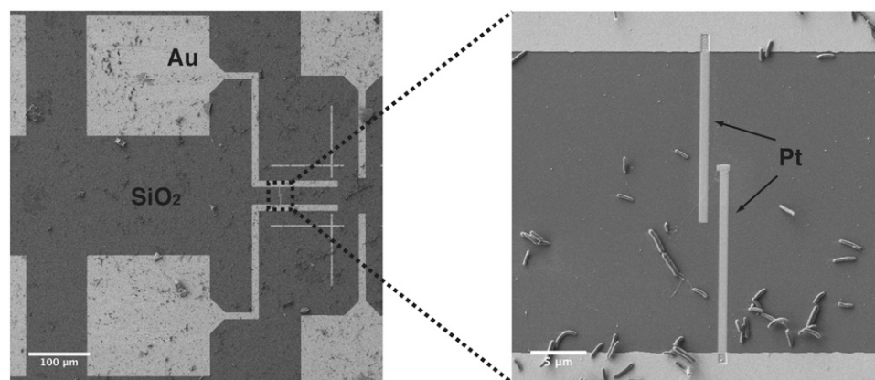
Fig. 1. Contacting individual bacterial nanowires with nanofabricated Pt electrodes. SEM images showing the geometry of the prefabricated Au contacts on \text{SiO}_2/\text{Si} . The zoom-in shows the FIB-deposited Pt contacts addressing a bacterial nanowire emanating from a S. oneidensis MR-1 cell.
