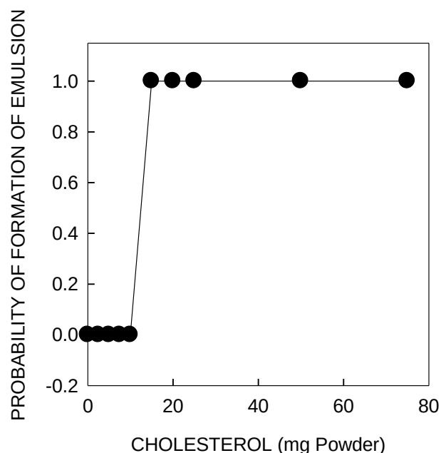
Figure 5 Effect of Cholesterol Concentration on the Formation of PFDC Emulsions
