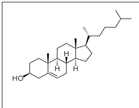
Figure 4A: Cholesterol Molecular Structure
