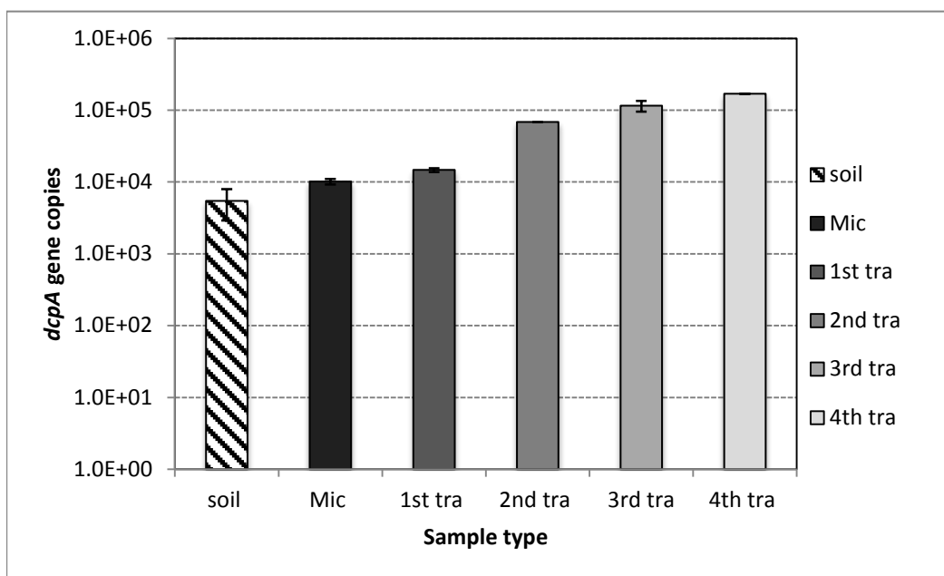
Figure 3.6. Application of the TaqMan-based qPCR assay for the Dhc 16S rRNA gene and the dcpA gene in Third Creek sediments and dechlorinating enrichment cultures. Top panel: Average dcpA copies per mL of culture (RC and KS enrichments); also indicated are the average 16S rRNA gene copies determined with qPCR. Bottom panel: Average dcpA copies per g of Third Creek sediment (bar on left labeled “soil”) and average dcpA copies per mL in microcosms (mic) and transfer cultures (tra). Error bars indicate the standard deviations of triplicate qPCR reactions and duplicate DNA extractions.
