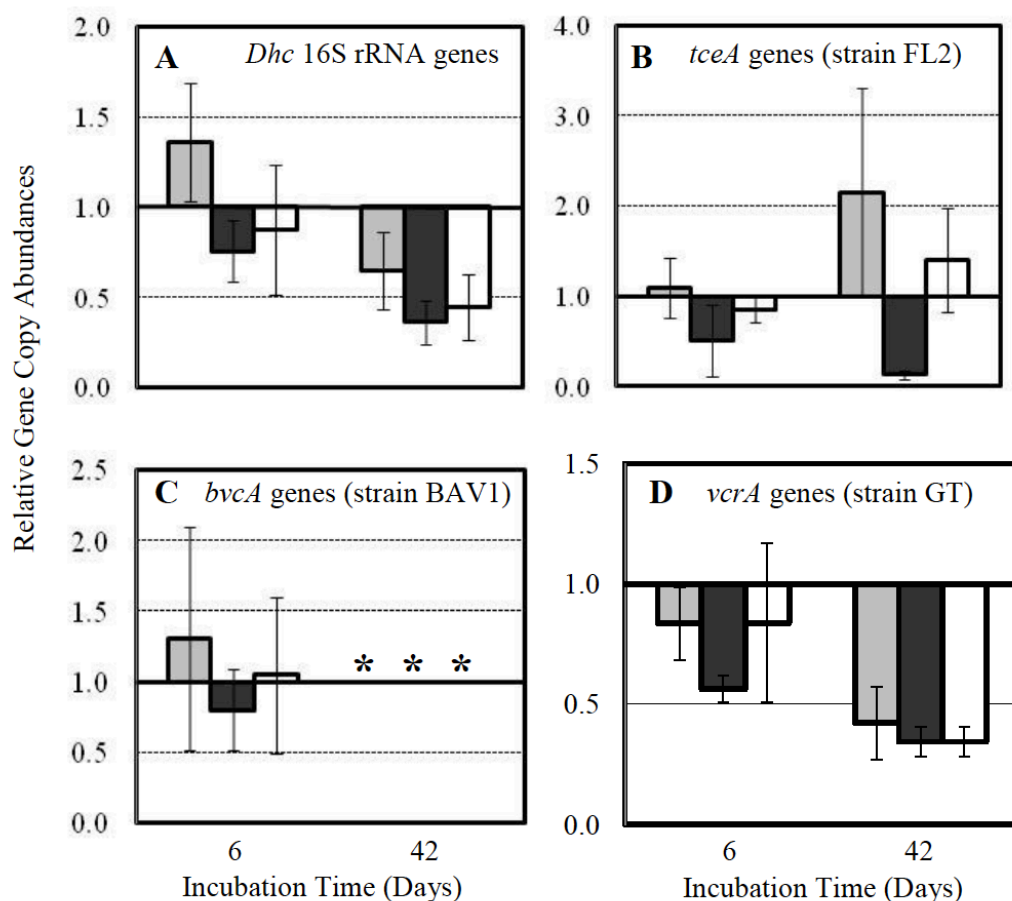
Figure 4.8. Dhc gene copy abundances in cultures incubated at 35°C (gray bars), 40°C (black bars), and in starved control cultures incubated at 30°C (white bars). Abundances of Dhc 16S rRNA (A), tceA (B), bvcA (C), and vcrA (D) gene copies were normalized to quantities measured in cultures incubated at 30°C and amended with PCE. The asterisks indicate that the bvcA gene was below the detection limit of 9.5 \times 10^3 gene copies per mL culture fluid in cultures incubated at 35 and 40°C and in starved control
