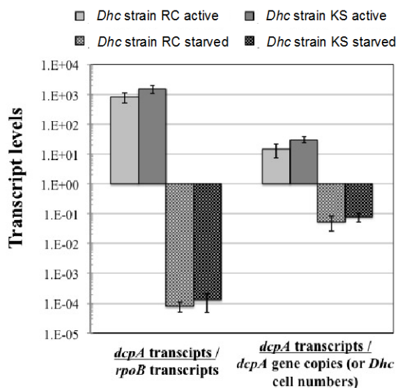
Figure 2.11. Gene expression levels in the 1,2-DCP-dechlorinating cultures RC and KS. dcpA transcript levels were normalized to rpoB or to dcpA gene copy numbers. Triplicate qPCR assays were run for each sample and final values represent the average of at least three biological replicate cultures. The error bars depict the standard error.
