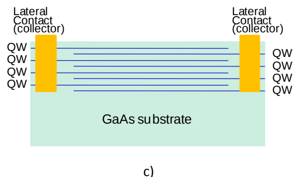
FIG. 1 Quantum Structures for Tunable Detectors. a) Structure I, b) potential profile of structure I, c) Structure II
