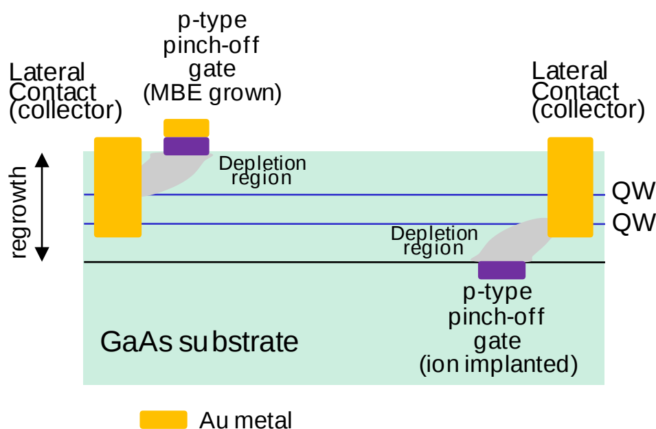
Fig. 2. Device with two quantum wells and p-type doping in the pinch-off gates.
