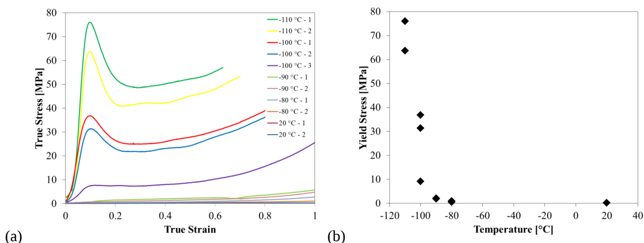
Figure 49. HTPB (a) true stress-true strain and (b) yield stress behaviour as a function of temperature ( -110 – 20^{\circ}\text{C} ) at a rate of 10^{-2}\text{ s}^{-1} . Note: for (b) true stress data at 0.1 true strain is reported above -80^{\circ}\text{C} .
