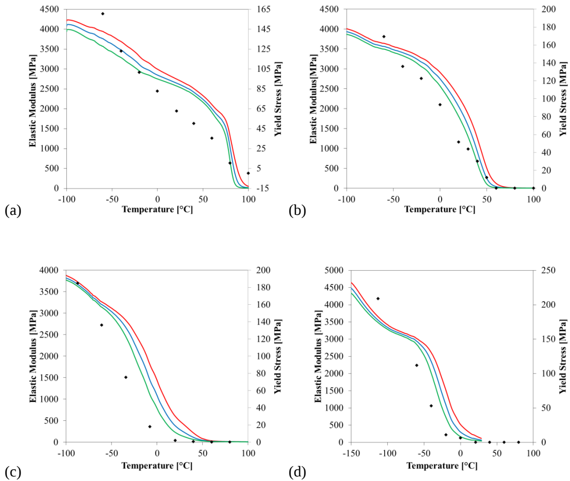
Figure 22. DMTA data for PVC (a), PPVC-2 (b), PPVC-4 (c), and PPVC-6 (d) at 0.035 \text{ s}^{-1} (1 Hz – green), 0.35 \text{ s}^{-1} (10 Hz – blue), and 3.5 \text{ s}^{-1} (100 Hz – red) with yield stress data at 10^{-2} \text{ s}^{-1} superposed.
