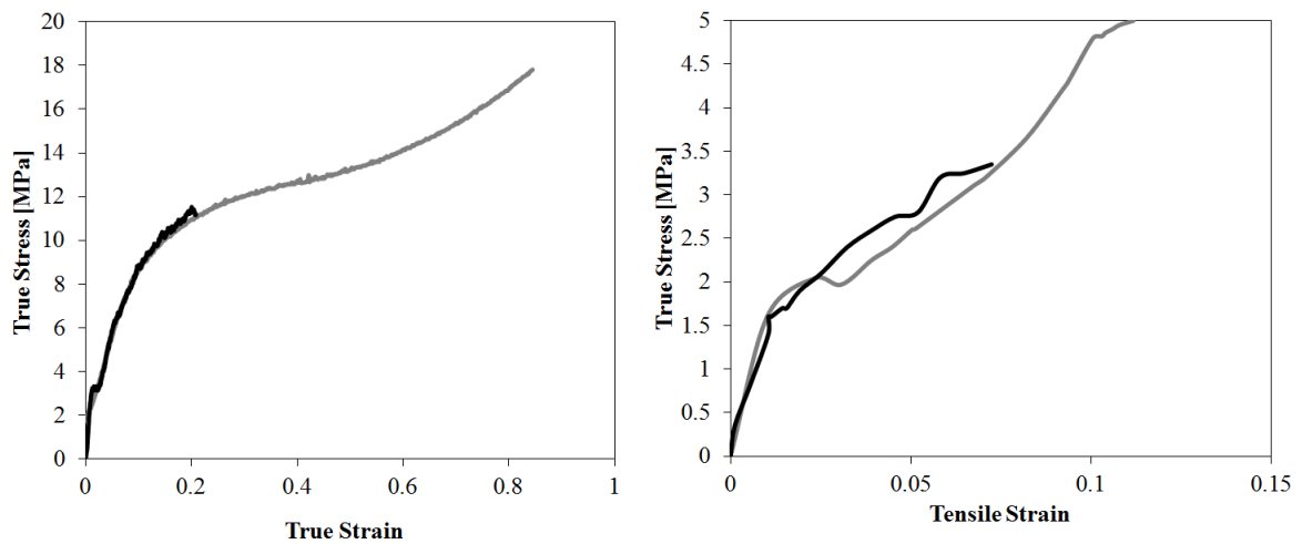
Figure 55. (a) PBS true stress-true strain behaviour in uniaxial compression at 1250 \text{ s}^{-1} at 20 \text{ }^{\circ}\text{C} : experiment (black) and experimental simulation (grey) at -45 \text{ }^{\circ}\text{C} . (b) PBS true stress-true strain behaviour in tension at 850 \text{ s}^{-1} at 20 \text{ }^{\circ}\text{C} : experiment (black) and experimental simulation (grey) at 45 \text{ }^{\circ}\text{C} .
