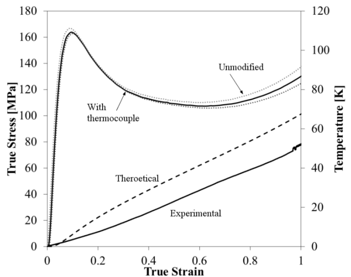
Figure 61. PMMA true stress-true strain behaviour using the foil sandwich method, and corresponding temperature rises (experimental – solid line; theoretical – dashed line) at 0.1 \text{ s}^{-1} . Representative true stress-true strain behaviours of unmodified PMMA at 0.1 \text{ s}^{-1} are included for comparison (grey dots).
