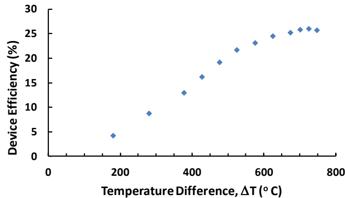
Figure 6. Measured heat-to-electrical conversion efficiency of optimized 3-stage TE device, showing a peak efficiency of 26%, a world record, for a \Delta T of 750^{\circ}\text{C} .
