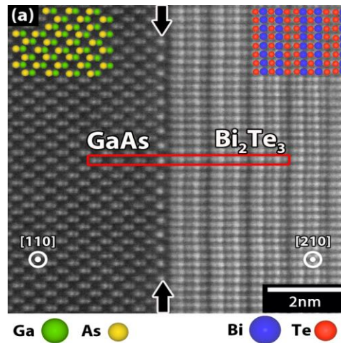
Figure 8. TEM image of atomic layer interface between \text{Bi}_2\text{Te}_3 and \text{GaAs} , showing formation of a thin \text{Ga}_2\text{Te}_3 interfacial layer that enables epitaxial growth of \text{Bi}_2\text{Te}_3 on \text{GaAs} .
