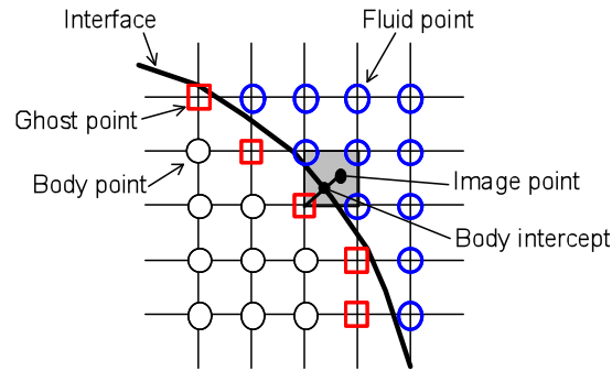
Figure 5: Schematic of the immersed boundary method
