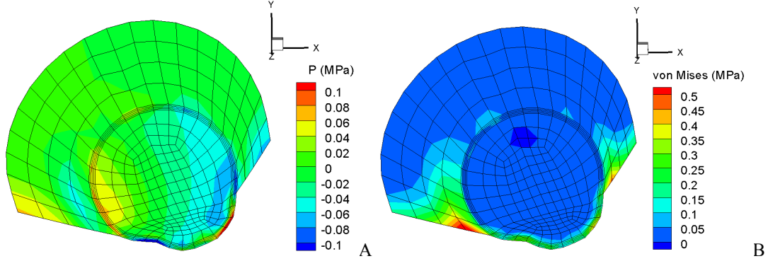
Figure 17: (A) Maximum pressure in the transverse plane of the orbit for case 2. Distortion of the globe due to the blast wave is shown by the deformed mesh. (B) von Mises stresses shown in the transverse plane, which is the largest in the extra-ocular tissue.
