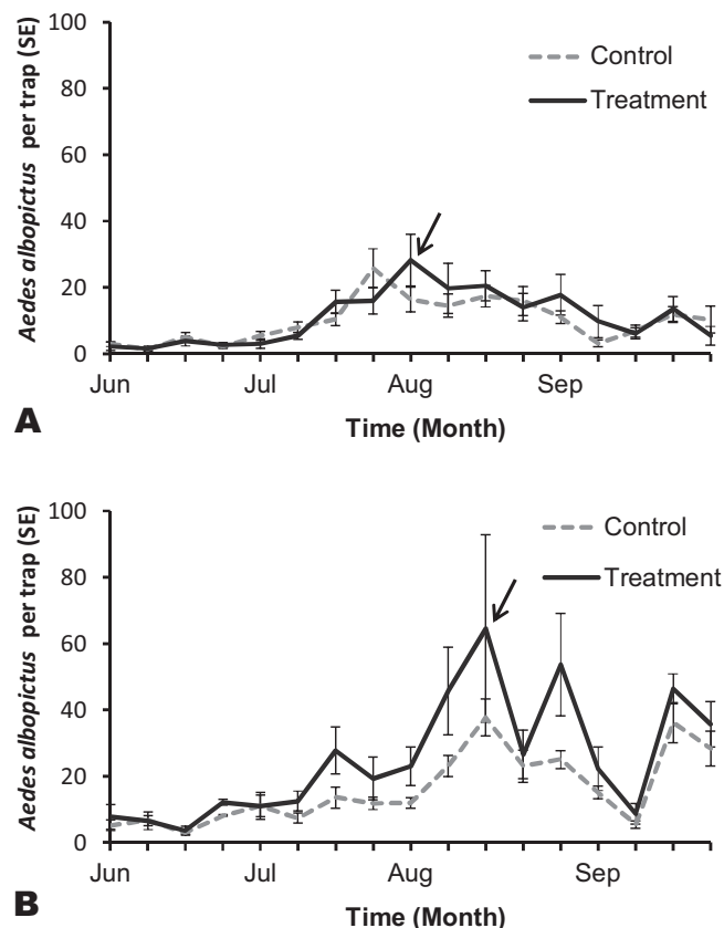
Fig. 6. Weekly population density of adult Aedes albopictus measured by BGS traps at area-wide treatment area (Keyport, NJ, USA) and control area (Union Beach, NJ, USA) during 2010 (A) and 2011 (B). Arrow indicates direct treatment schedule.
