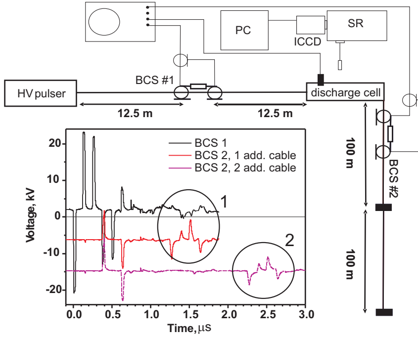
Figure 2.2: Scheme of the experimental setup and typical shape of signals from the back current shunts. Circles 1,2 designate additional reflections from the cable end used to excite \text{N}_2(\text{C}^3\Pi_u) emission (see text for the detailed explanations).
