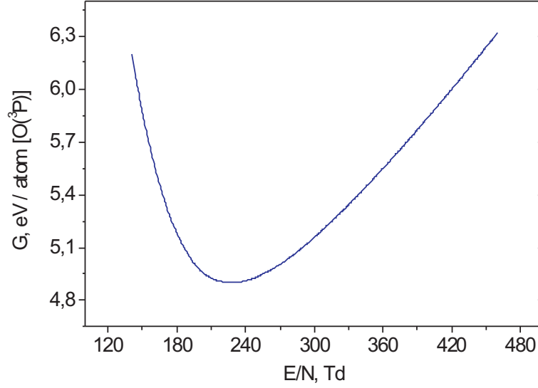
Figure 3.14: Energy efficiency of O( 3 P) production in air, G , as a function of a reduced electric field E/N .
