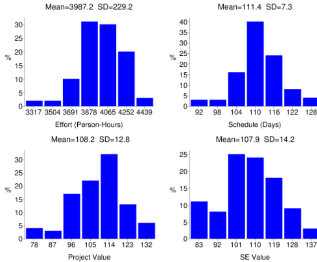
Figure 5. Example Monte Carlo results.
