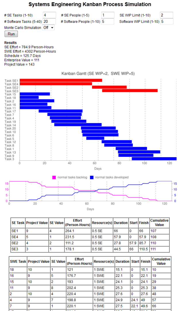
Figure 2. Project simulation example (SE WIP=2, SWE WIP=5).
