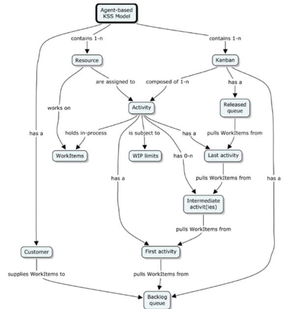
Figure 6. Agent-based model of kanban-based scheduling system.
