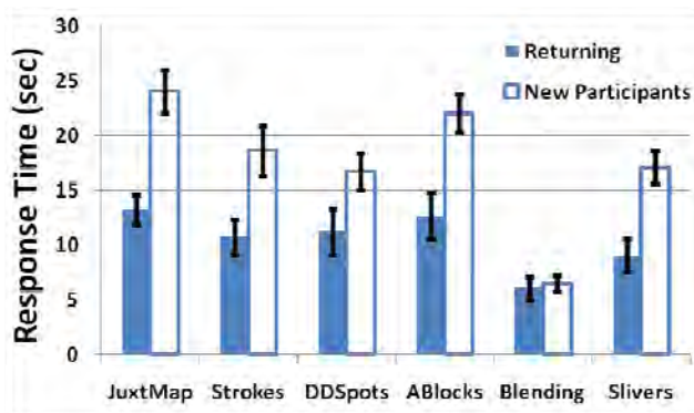
Figure 7: The main effect of visual technique on response time was largely due to the speed with color blending.
