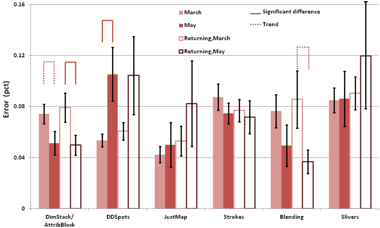
Figure 6: Performance changes with regard to error, separated by visualization technique, included improvement for attribute blocks over dimensional stacking and a loss of performance for DDS. Filled bars compare all data of the two studies; outlined bars compare performance of only subjects who participated in both. Coupling bars indicate significant differences (solid) or trends (dashed).
