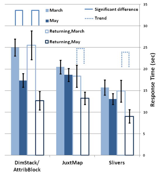
Figure 9: Comparison of response times between the two experiments showed a significant decrease in the response time needed for attribute blocks compared to dimensional stacking, and trends for decreased response times for juxtaposed maps and oriented slivers.
