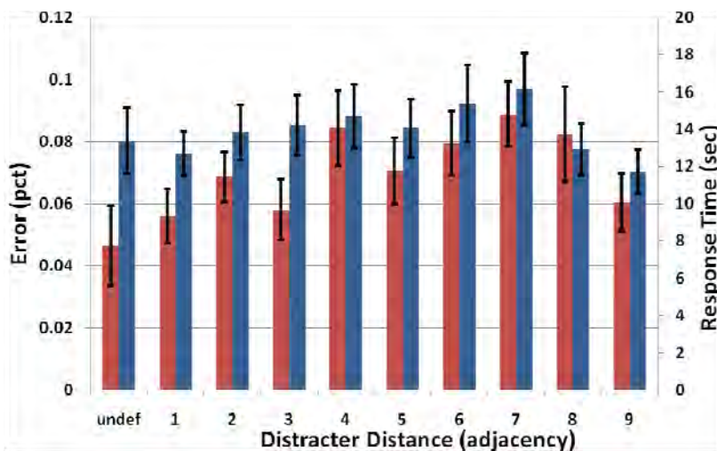
Figure 5: Distracter distance had a main effect on both error (light red bars) and response time (dark blue bars); users were more accurate when there was no distracter or it was close to the target, but fastest when a distracter was very distant. In all result graphs, error bars indicate the standard error, red hues indicate error, and blue hues indicate response time.
