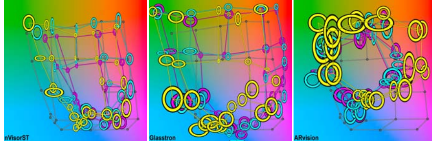
Fig. 6 The perceptual matching showed the color distortion in the nVisorST ( left ), Glasstron ( center ), and ARvision ( right ). The same three visual conditions are graphed with the same colors as in Figure 5. All data should be compared to the measured color gamut of the reference monitor, again mapped by the gray graph. In this figure and Figure 5, the CIELAB domain is represented by the L=65 slice with a and b in [-100,100] . This portion of the domain is also depicted in Figures 7 and 8 and thus may be used to help compare the data in all four graphs.
