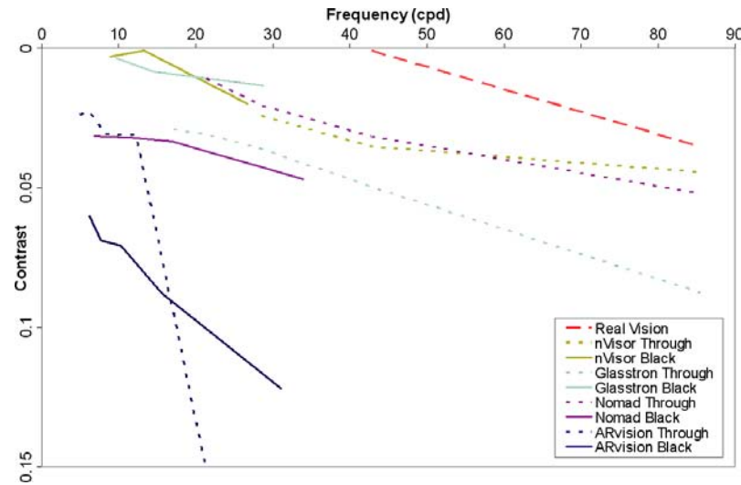
Fig. 4 The sampled CSF for four head-worn AR displays. The size of the target decreases as frequency (measured by cycles per degree) increases to the right. The contrast is typically graphed with lower contrast at the top of the vertical axis. In this test, the nVisorST performed well in both the see-through and graphical cases, the Glasstron provided sharp graphics, the Nomad provided clear see-through, while the ARvision struggled in both cases.
