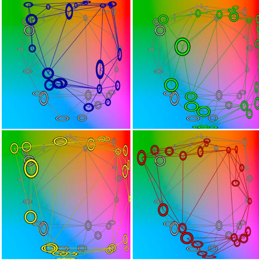
Fig. 8 The perceptual matching showed the color distortion in the nVisorST for four canonical chromatic backgrounds of solid color: Blue (upper left), Green (upper right), Yellow (lower left), and Red (lower right). Each graph is shown on CIELAB space and includes a gray reference grid of the matching as completed with no mediation by any AR display.
