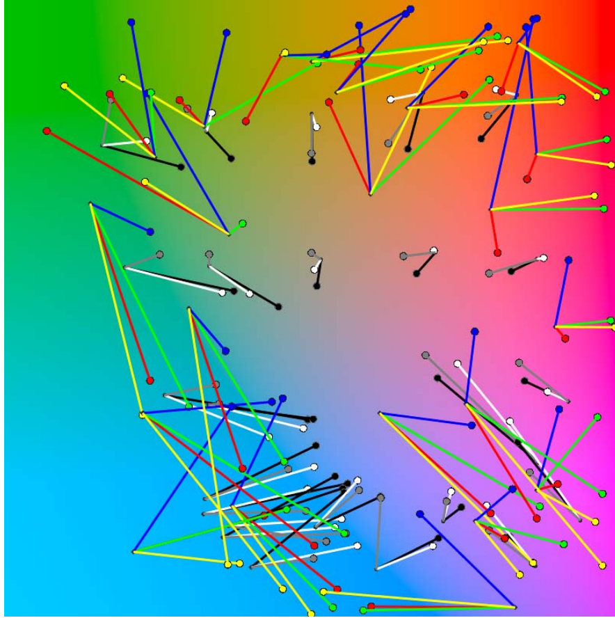
Fig. 9 In comparing the direction and magnitude of the color matching error under the various background conditions for the two color matching experiments, we see a few patterns emerge in CIELAB color space. The reference color is denoted by small, dark gray circles with no outlines, whereas the circles with outlines represent the mean color error ( \Delta E , represented by distance and angle in color space) in user matching. The achromatic circles with gray or black outlines indicate the black or white backgrounds according to their inner color, with the gray inner circles with black outlines indicating the see-through condition. In the first test, we used a set of 24 reference samples. The colored circles with black outlines indicate the colored backgrounds (red, green, blue, and yellow) from the second experiment, which used a new set of 22 reference samples.
