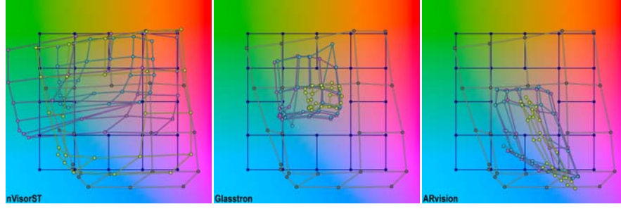
Fig. 5 Objective measurements of color distortion in the nVisorST ( left ), Glasstron ( center ), and ARvision ( right ) as determined by spectrophotometer measurements. Three visual conditions were of interest: see-through (yellow graphs) – a misnomer for the video overlay ARvision, but still a convenient label, graphics-on-black background (magenta graphs), and graphics-on-white background (cyan graphs). The see-through data should be compared to the measured color gamut of the reference monitor that was the real-world background; this data is mapped by the gray graph. The blue reference grid gives the definitions in CIELAB space of the colors sent to the displays.
