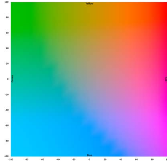
Fig. 3 The CIELAB space aimed to both mimic the physiological measurements of the eye and form a perceptually uniform color space. This slice at L = 65 shows the a axis running from green (left) to red (right) and the b axis running from blue (bottom) to yellow (top). The origin of the ab plane is the gray point in the center of this plot. The portion of the space shown here ranges from -100 to 100 in both a and b and corresponds to the portion drawn in later graphs.
