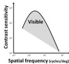
Fig. 1 The canonical shape of the contrast sensitivity function, graphed as a function of spatial frequency for size and contrast threshold for sensitivity.
