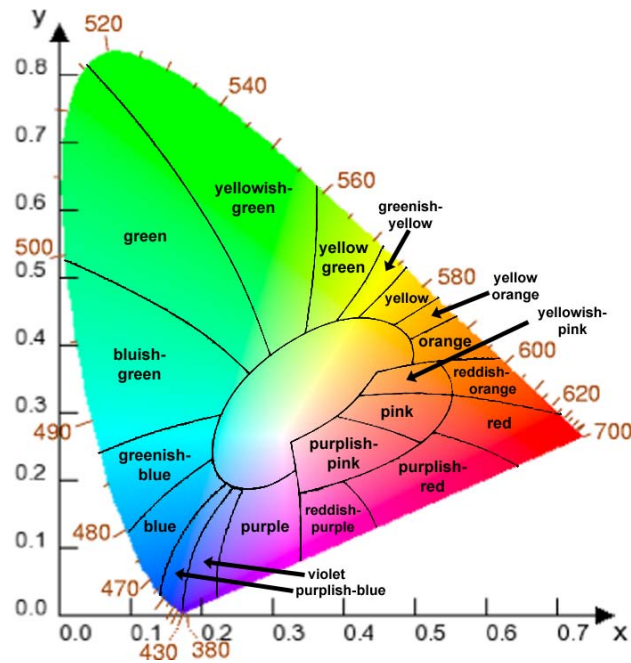
Fig. 2 Names may be superimposed on the regions of a color space, such as the 1931 CIE chromaticity diagram seen here. However, some of these names are far from common usage, and individuals will exhibit differences in the names.
