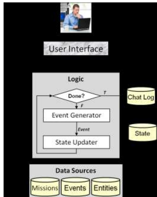
Figure 3: A diagram showing the framework of the logic for the chat generator.
