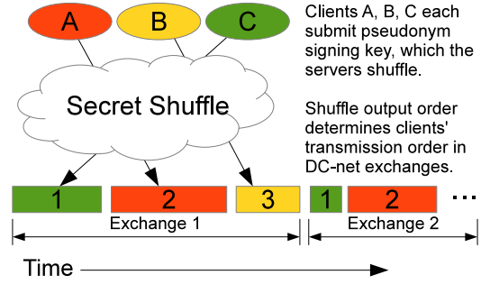
Figure 2: DC-nets scheduling via a verifiable shuffle
