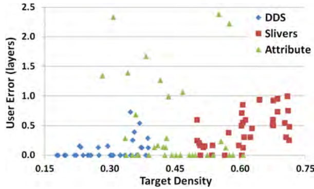
Fig. 8. A scatterplot of user error versus target density for each trial question (averaged over all users) shows that merely increasing density did not improve performance. Not shown is the ratio of density between target and distraction. The ratio appears to offer a better explanation for improved performance.
