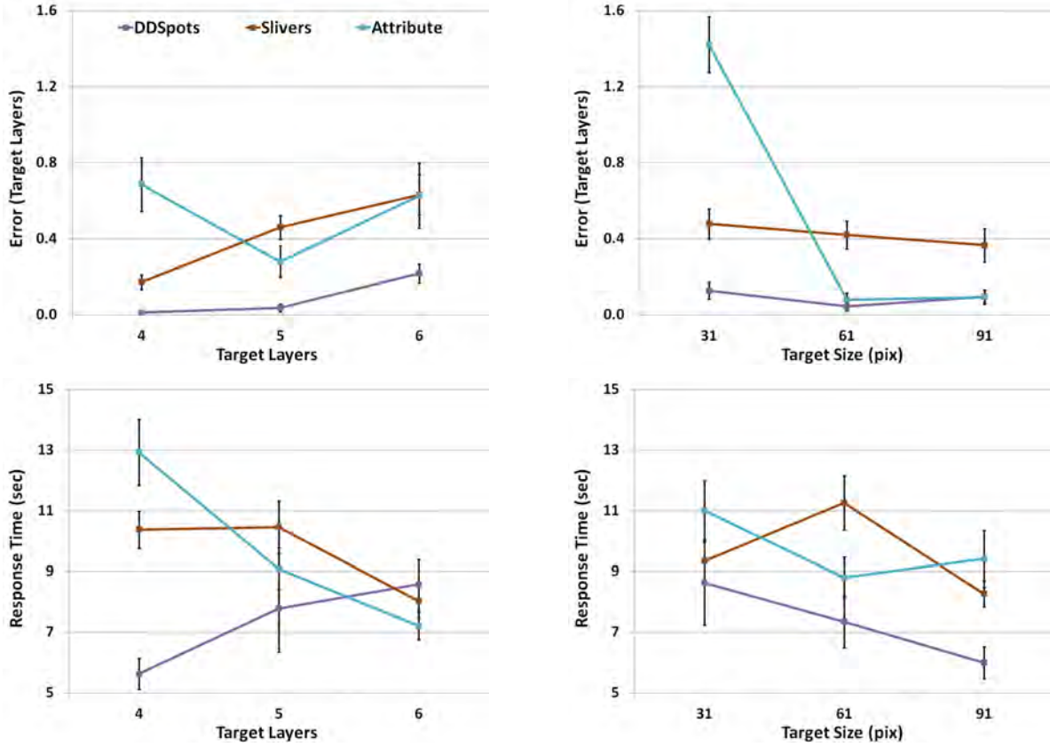
Fig. 7. Significant interactions were found between MVV technique and number of target layers for both error (top left) and response time (bottom left). Significant interactions were also found between MVV technique and target size for both error (top right) and response time (bottom right). Error bars in all graphs indicate one standard error unit.
