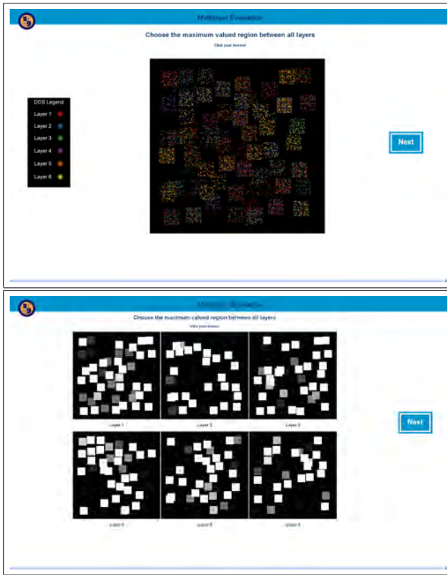
Fig. 5. Screen-captured images for the (top) Data-driven Spots and (bottom) Juxtaposed Layers techniques.
