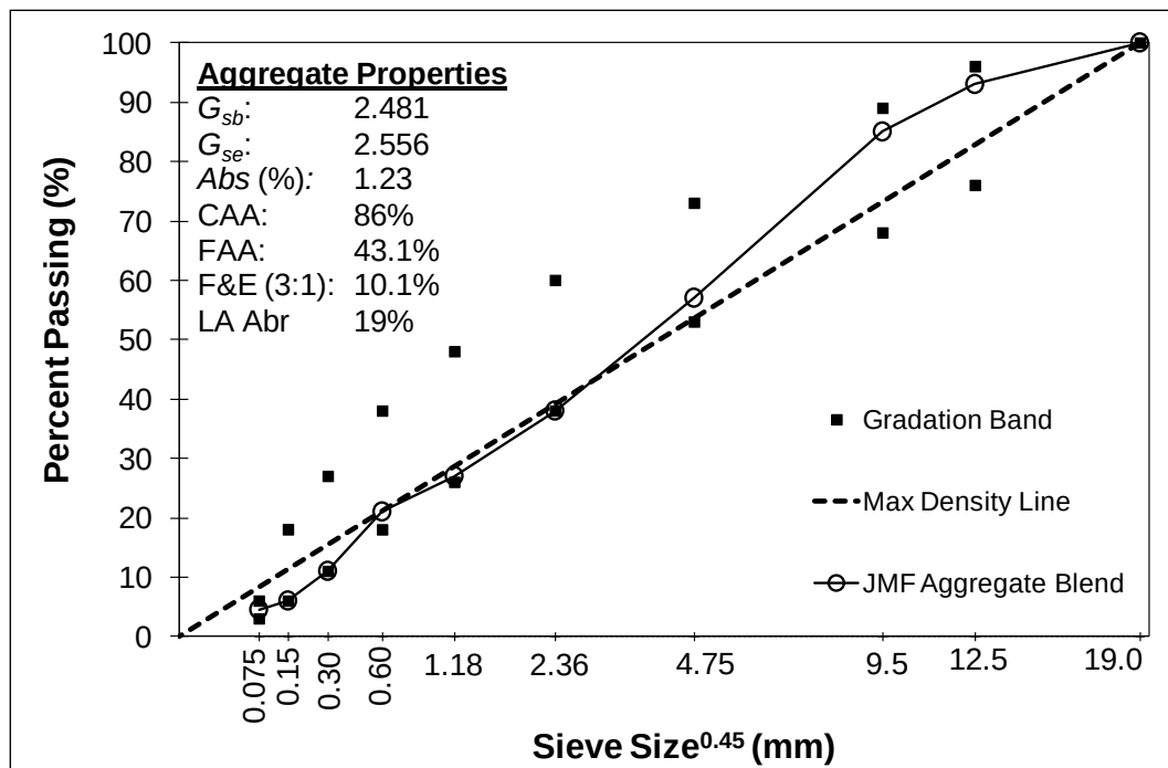
Figure 27. Aggregate blend for Columbus AFB base mixture.
