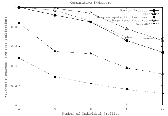
Figure 4. Comparative Results for discrimination between 2-10 users using weighted F-measure
