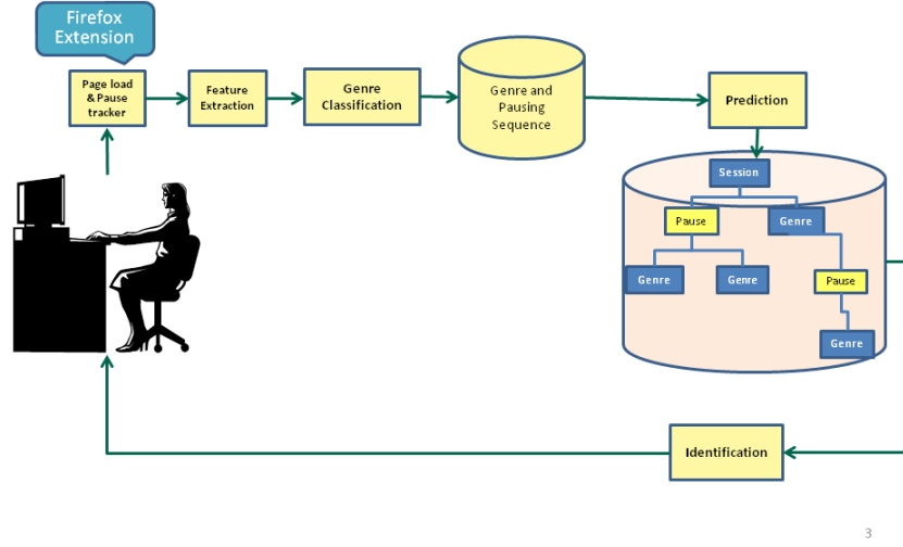
Figure 1. Web behavior attribution data flow
