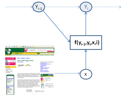
Figure 3. CRF feature linking temporal states y_{i-1} and y_i with document features x .
