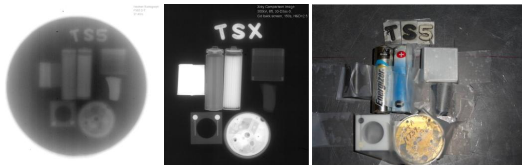
Figure 1: Early P385 Neutron Image vs. a comparable X-ray radiograph and visual setup
