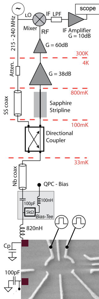
Fig. 2. Fast readout electronics based on high-Q resonant circuit.
