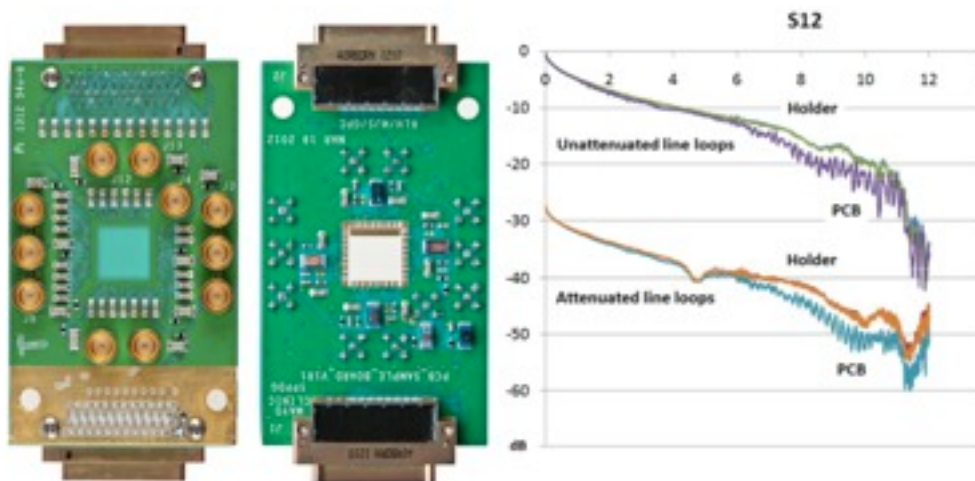
Fig. 3. High-bandwidth circuit boards designed for spin qubits.
