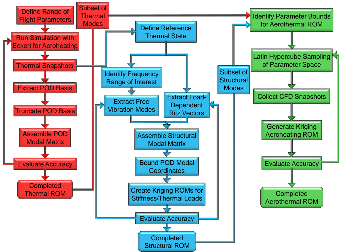
Figure 6.3: Flowchart of aerothermoelastic ROM generation process.
