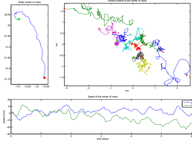
Figure 1: Upper left: path of the center of mass (green dots indicate start of track). Upper right: drifters' positions relative to the center of mass. Bottom: center-of-mass velocity.
