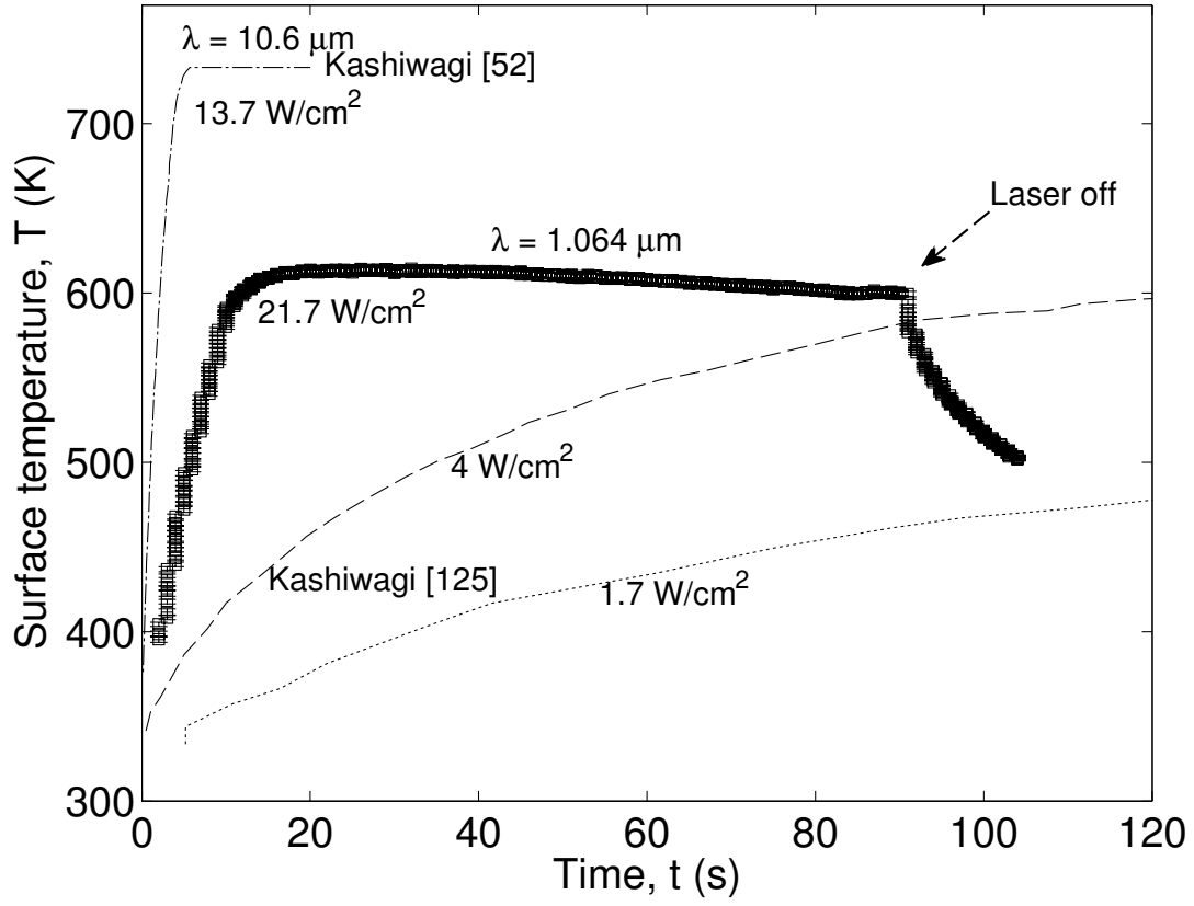
Figure 26. Temporal evolution of surface temperature irradiated with a 1.06 \mu\text{m} Nd:YAG laser at 21.7 \text{W}/\text{cm}^2 ( \square ), compared against irradiated PMMA surfaces with a 10.6 \mu\text{m} \text{CO}_2 laser at 13.7 \text{W}/\text{cm}^2 (--) from [52] and electrically heated at 4 \text{W}/\text{cm}^2 (--) and 1.7 \text{W}/\text{cm}^2 (··) from [125].
