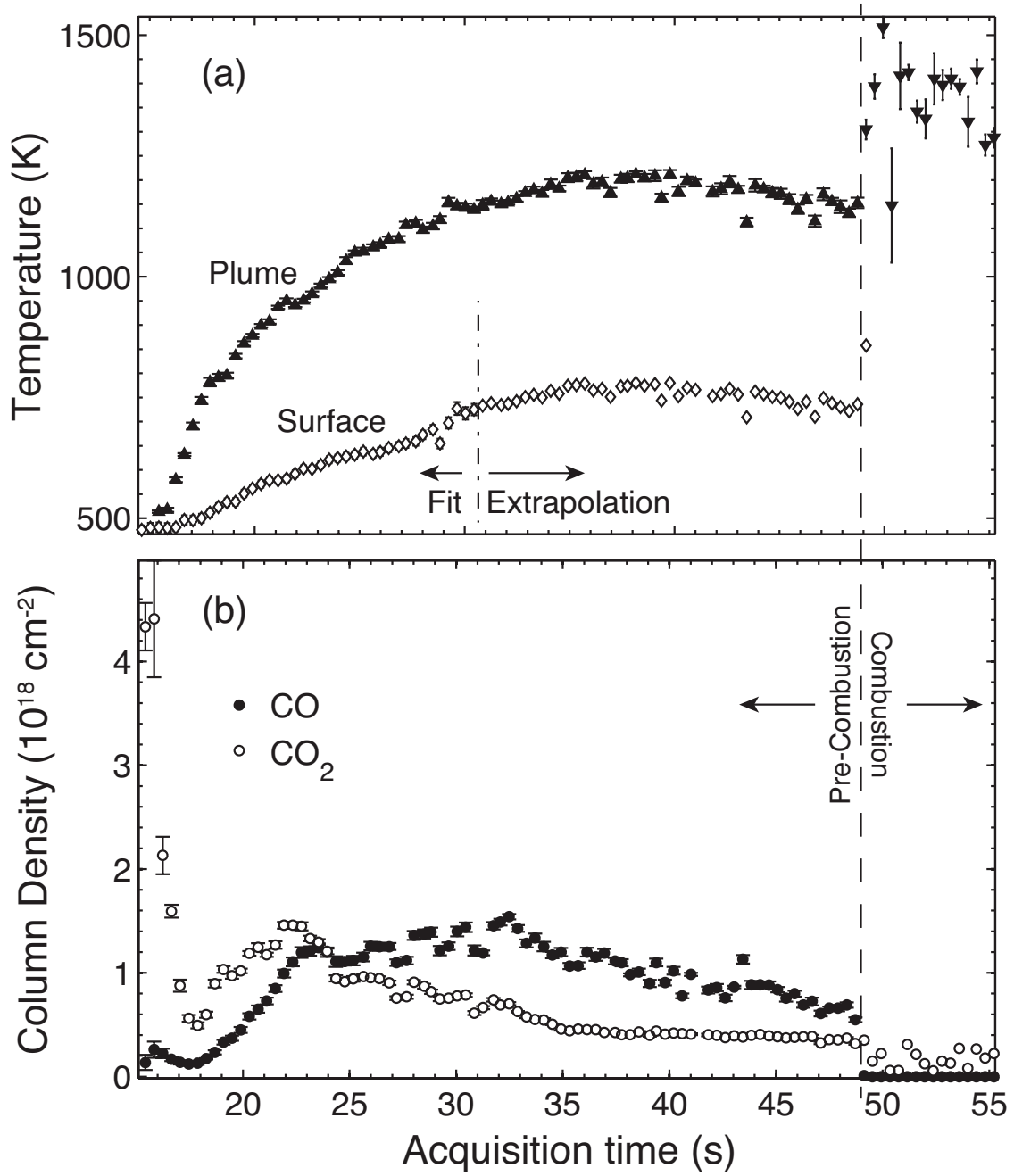
Figure 12. (a) Temporal evolution of plume and surface temperature and (b) temporal CO, CO 2 column densities for t \geq 15 s. The pre-combustion data is for (x,y) = (1.8 \text{ mm}, 12.6 \text{ mm}) and the combustion data is reported for (x,y) = (6.3 \text{ mm}, 12.6 \text{ mm}) .
