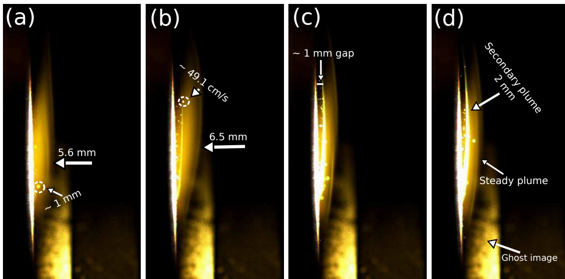
Figure 38. High-speed visible imagery of steady-state diffuse plume and secondary plume of laser irradiated graphite at 777 W/cm 2 at (a) 54.48 s, (b) 54.53 s, (c) 54.58 s and (d) 55.60 s with a 0.14 mm/pixel spatial resolution. The ghost image is due to an out-of-focus image of a bright source in the field-of-view of the camera.
