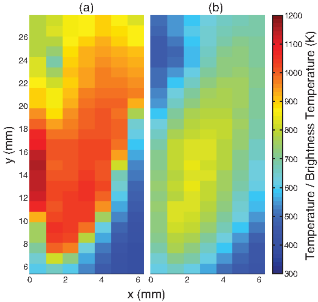
Figure 10. Spatial maps of the: (a) Fit plume temperature, T obtained from the LBLRTM calculation at t = 24 s, (b) Brightness temperature that correspond to a hot CO 2 peak at 2295 cm -1 .
