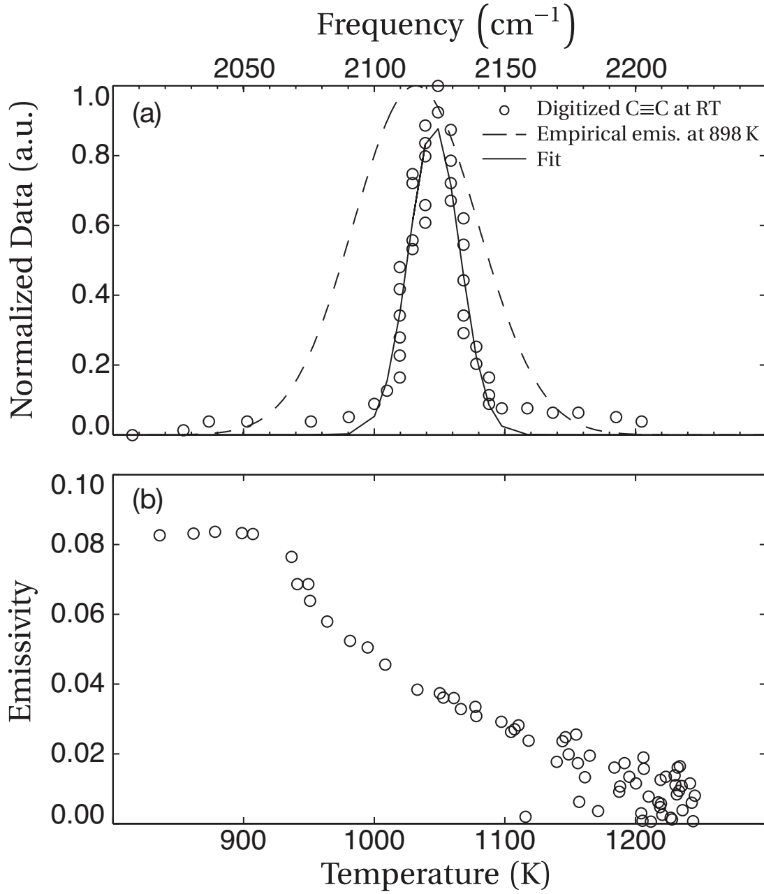
Figure 9. (a) Comparison of (o) \text{-C}\equiv\text{C-} spectra from 1-octyne at room temperature (RT) [105] with (---) empirical emissivity of equation (3) for the pixel (x,y) = (1.88 mm, 12.6 mm) at 24 s, with temperature T = 898 K, and (b) peak amplitude of empirical emissivity, A(\nu=c_2) , as effective plume temperature increases.
