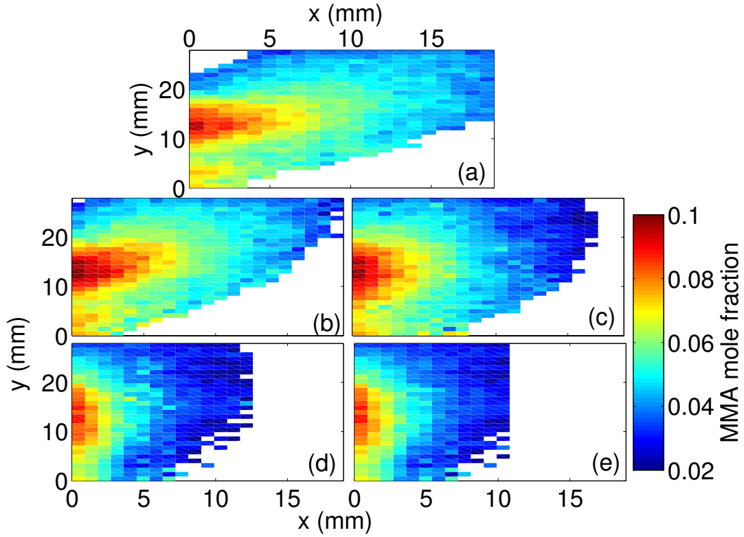
Figure 28. Time averaged spatial maps of MMA concentrations of the boundary-layer plume from laser irradiated PMMA at (a) 21.7 \text{ W/cm}^2 , (b) 17.4 \text{ W/cm}^2 , (c) 13.0 \text{ W/cm}^2 , (d) 8.7 \text{ W/cm}^2 and (e) 4.3 \text{ W/cm}^2 .
