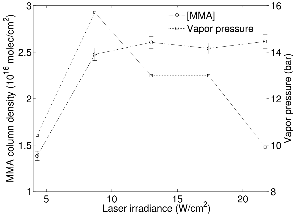
Figure 31. Spatially averaged MMA surface column density (O) and MMA vapor pressure ( \square ) along the surface-boundary layer in the vertical direction ( 9 \text{ mm} \leq y \leq 16.2 \text{ mm} ) for irradiances between 4.3 to 21.7 W/cm 2 .
