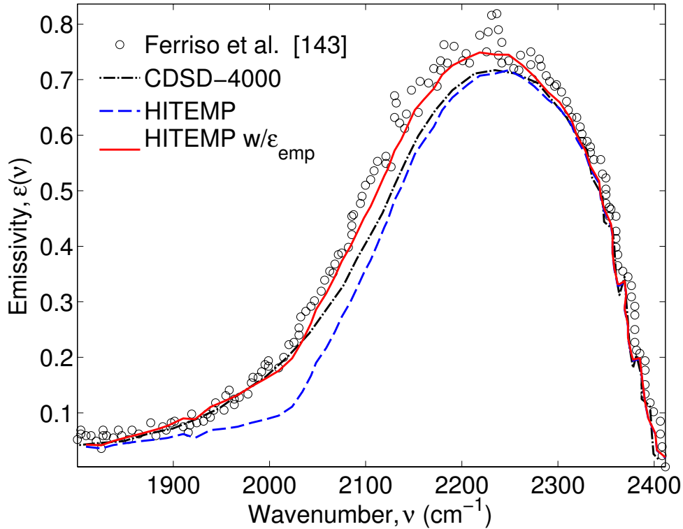
Figure 40. Experimental [143] and simulated emissivity of \text{CO}_2 , \text{H}_2\text{O} and \text{CO} at 2850 K in the 4.3 \mu\text{m} region.
