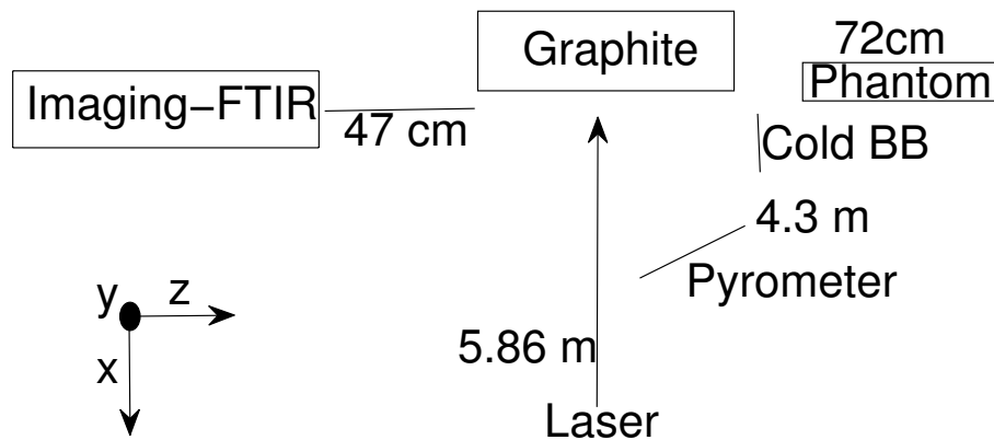
Figure 33. Schematic experimental set-up.
