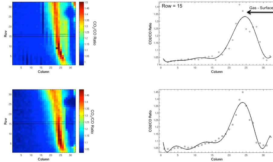
Figure 54. Ratio of CO 2 /CO spatial brightness temperature maps for unpainted (top left panel) and painted (bottom left panel) fiberglass composite. Plot of the CO 2 /CO ratio along all columns of row 15 for unpainted (top right panel) and painted (bottom right panel) fiberglass.
