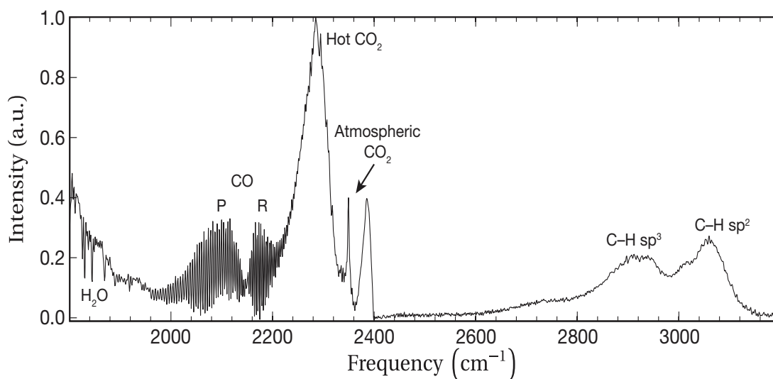
Figure 7. Normalized FTIR spectra for (x,y) = (1.8\text{ mm}, 12.6\text{ mm}) at 24 s.
