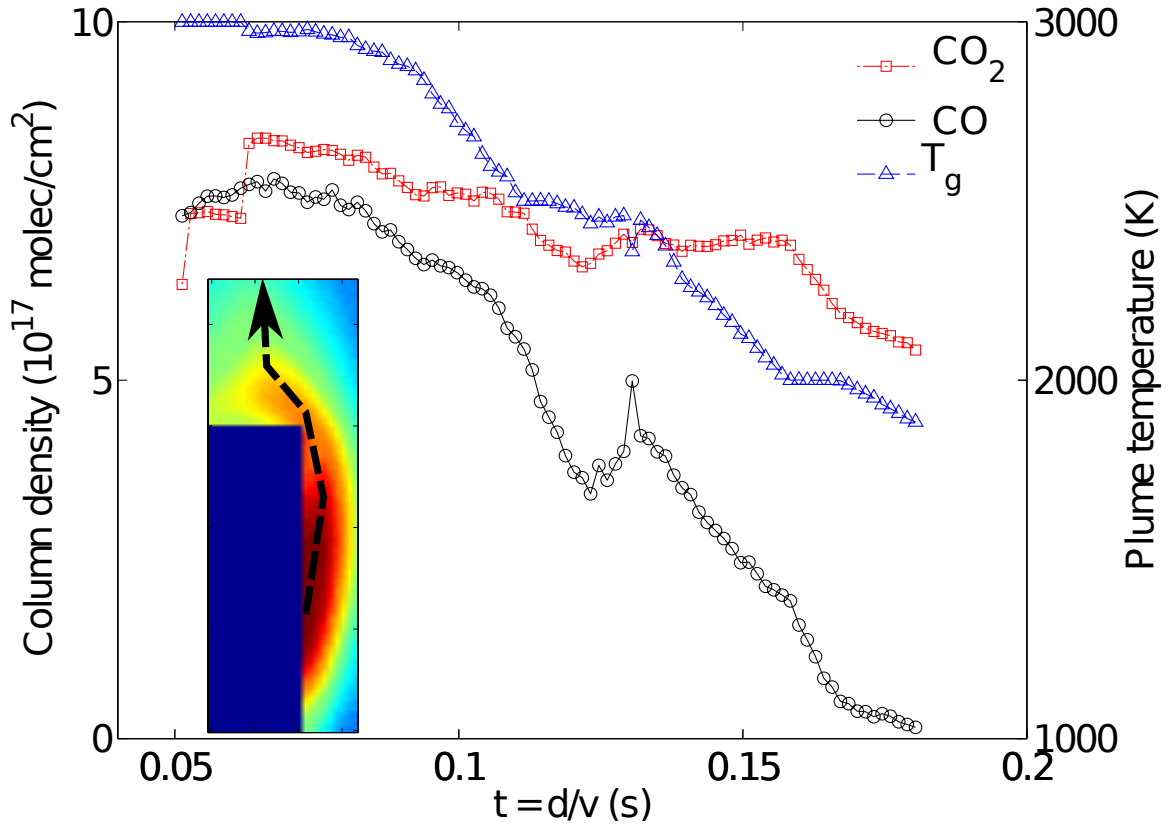
Figure 49. Profiles of gas-phase species column density and plume temperature along the buoyant driven boundary layer, with surface temperature at \sim 2500 K as a function of t = d/v . Inset: spatial plume temperature map with vector showing the path parallel to the surface along the boundary layer driven by the buoyant flow of the shown profiles.
