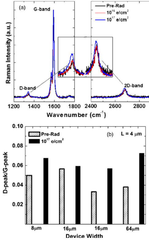
Figure 14: Raman spectra presented before and after irradiation (top), along with the D/G ratio as a function of channel width (bottom). Reproduced with permission from Francis et al. [3].
