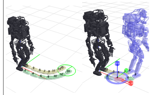
Left: Sequence of poses to generate motion path. Right: Navigation goal specifying destination pose.
