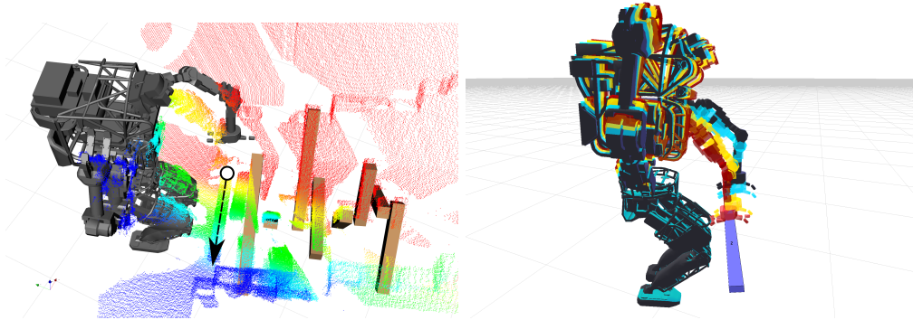
Figure 11: A fitting algorithm produces an affordance that can be used to plan a reach motion. Left: A line annotation defines a search region that is used by a segmentation algorithm to fit a 2"x4" board affordance to the 3D point cloud data. Right: An end-effector goal placed on the board affordance is used to compute a reaching plan.
