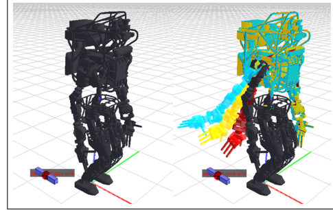
Left: End-effector goal specifying a 6-DOF pose constraint. Right: Gaze goal specifying an orientation constraint.
