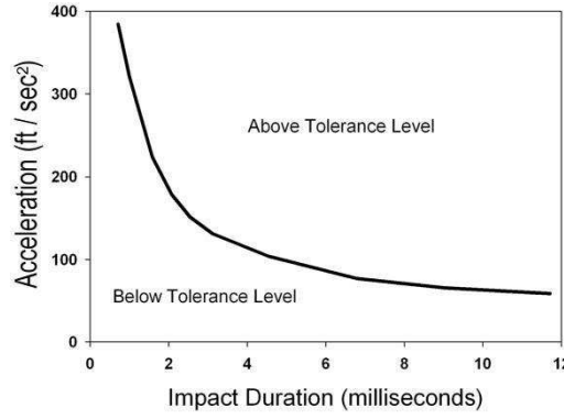
Fig. 1: Wayne State Tolerance Curve. [10]
