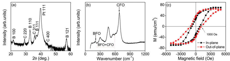
FIG. 1. (a) X-ray diffraction collected from the BFO-CFO nanocomposite thin film. The indexed peaks labeled B and C correspond to BFO and CFO, respectively; (b) Raman spectrum: arrows denote assigned Raman bands; (c) magnetic hysteresis loops for the in-plane and out-of-plane directions of BFO-CFO nanocomposite thin film measured at 300 K.
