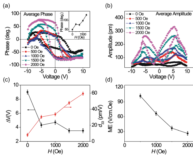
FIG. 4. The local ferroelectric switching characteristics in BFO-CFO nanostructures by the application of external magnetic field by VFM. (a) Average phase-voltage hysteresis loop: the inset shows the remanent phase change as a function of magnetic field; (b) average amplitude-voltage butterfly loop; (c) measured variation in hysteresis loop width and piezoelectric constant d_{33} as obtained from (a) and (b); (d) the ME coefficient as a function of H , calculated from experiment.
