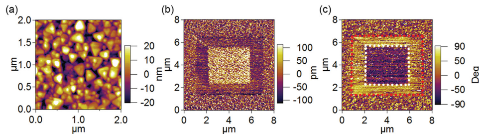
FIG. 2. (a) AFM topographic image ( 2 \times 2\text{ }\mu\text{m}^2 ): results are consistent with BFO nanoparticles embedded within pyramidal CFO nanopillars; (b) and (c) out-of-plane PFM (OP-PFM) amplitude and phase images taken after poling the nanocomposite film using +9 V ( 5 \times 5\text{ }\mu\text{m}^2 , outside frame) and -9 V ( 3 \times 3\text{ }\mu\text{m}^2 , inside frame). The poled area is denoted using dashed red lines to convey the change in contrast in both amplitude and phase images in accordance with switched ferroelectric domains.
