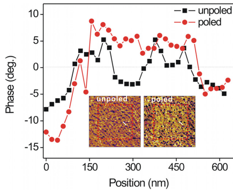
FIG. 3. Line profiles across CFO grains collected from MFM images. The insets are subsets of collected MFM images of the same area ( 3 \times 3 \mu\text{m}^2 , red frame) prior to (left) and following (right) electric-field poling, with the white lines denoting the traces from which the line profiles were extracted. The color map corresponds to a range of -5^\circ to +5^\circ . These representative results demonstrate that the applied electric field reorients the magnetization of CFO in some areas.
