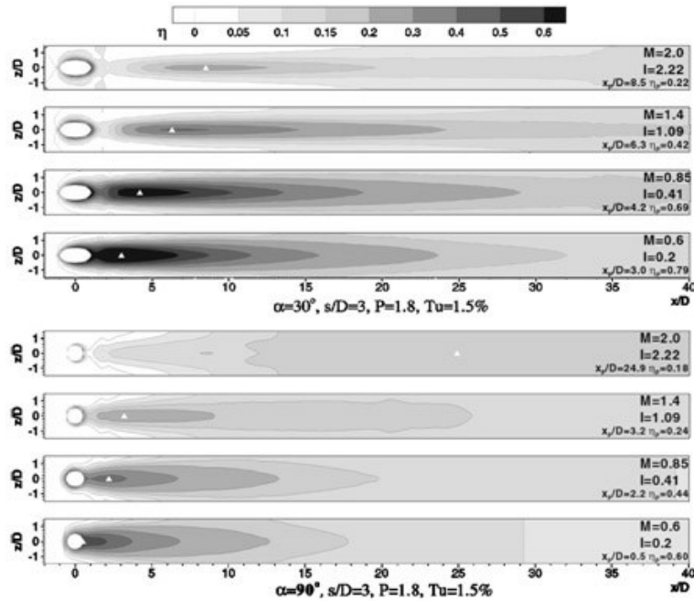
Figure 0.2: Effect of Injection Angle on adiabatic effectiveness [8]
