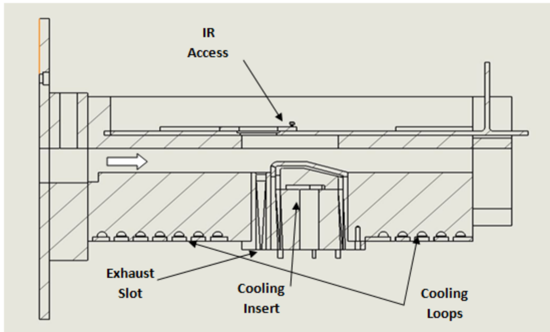
Figure A.2: Test Rig Side View
