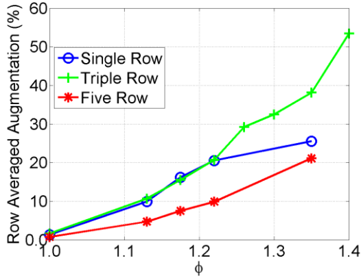
Figure 0.16: Robertson, \sigma vs. \phi , X/D = 20
