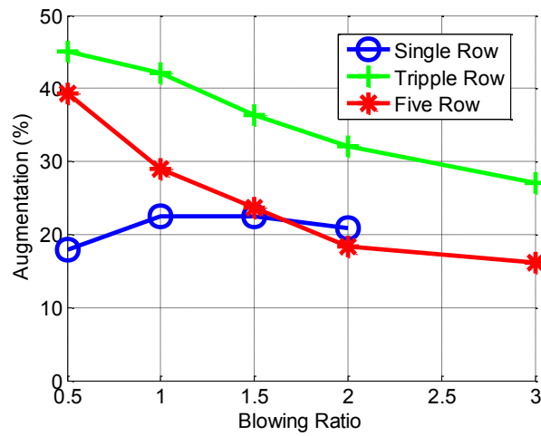
Figure 0.11: Shewhart, \sigma vs. M , X/D = 22
