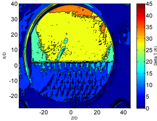
Figure 0.34: Temperature Difference, IR Image, M = 2.0 , \phi = 1.3
