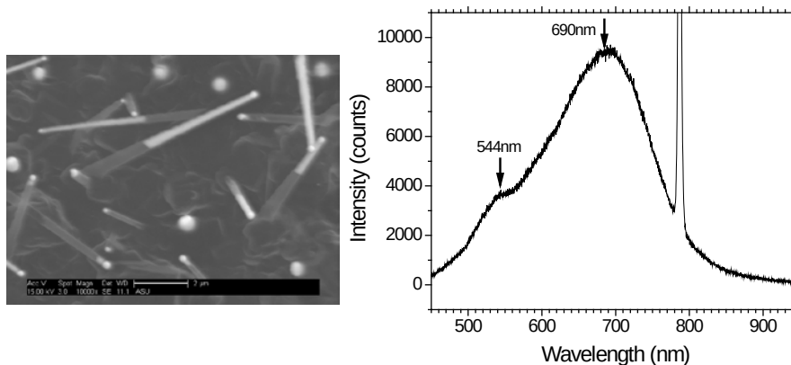
Figure 4: SEM (left) and PL (right) of PbS-CdS alloy nanobelts. The contrast change in the SEM indicates the heterostructures formed with alloys of two different compositions.
