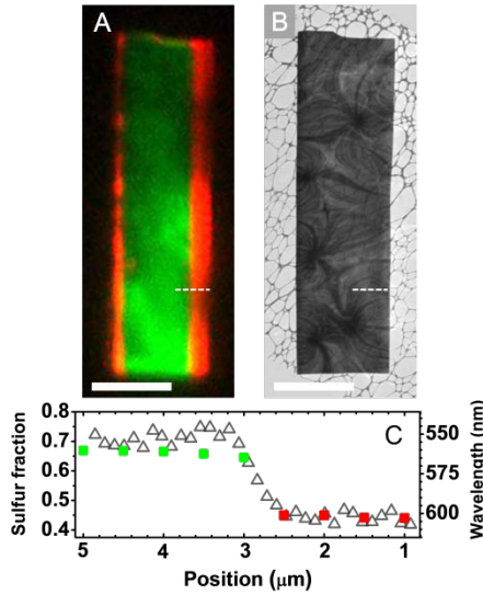
Figure 13 (A) Real-color PL image of a CdS/CdSe lateral heterostructure nanosheet excited by 405 continuous-wave laser. (B) TEM image of the same nanosheet. The scale bars in (A) and (B) are 10 \mu\text{m} . (C) Comparison of sulfur molar fraction between EDS scan (hollow triangles) and micro-PL scan (solid squares) along the white dashed line in (A) and (B).
