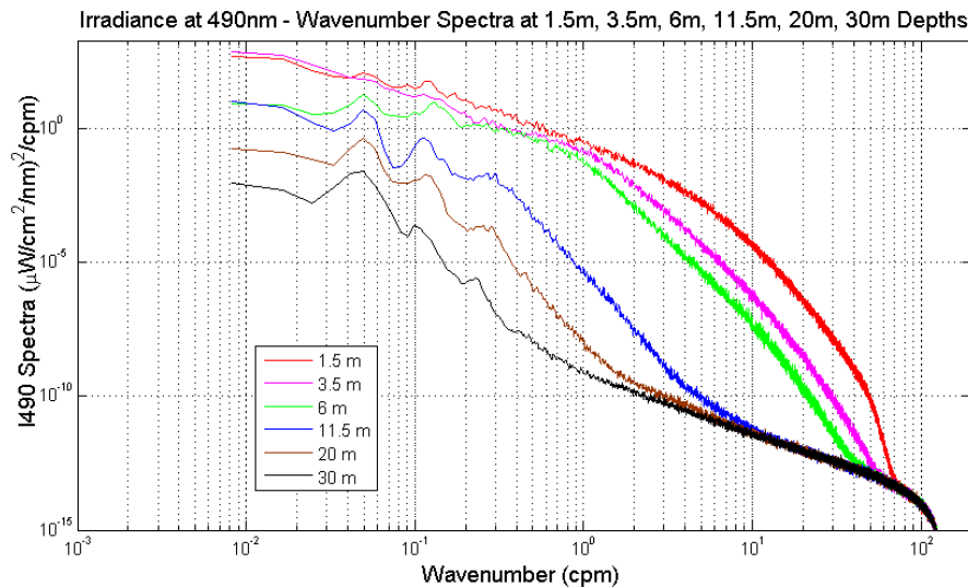
Figure 5. Shown is the wave number spectra at six depths for irradiance at 490 nm observed on Sep 20, 2009. Westerly winds were about 6 m/s and solar insolation varied from 650\text{ to }850\text{ W m}^{-2} during the observation. The fluctuations at shorter wave numbers decrease rapidly with depth.
