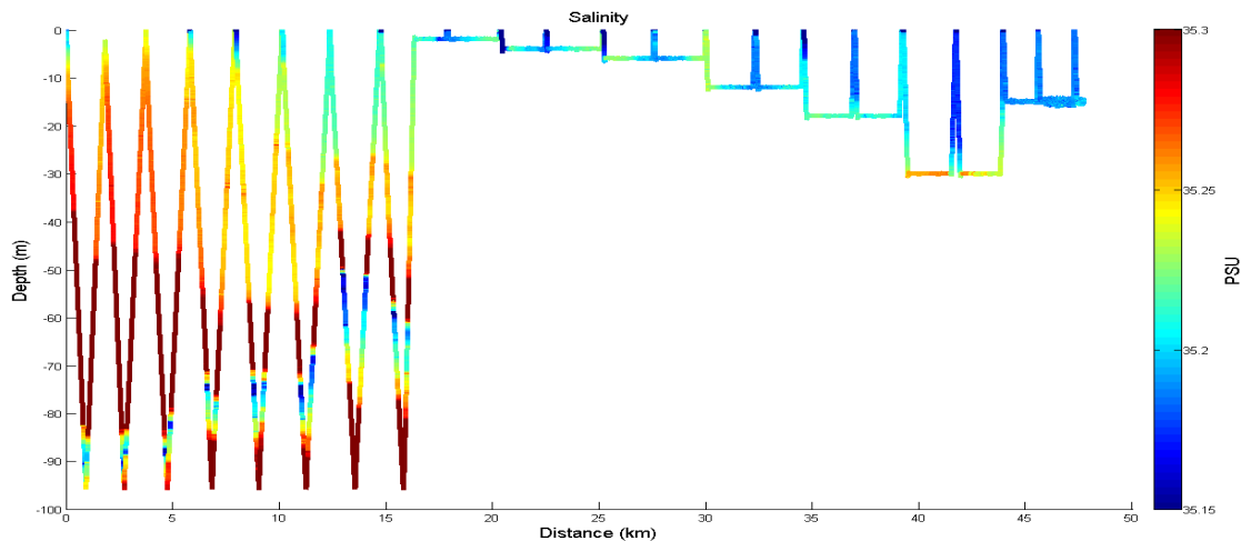
Figure 2. A trace of the salinity (color) as a function of depth (y-axis) and distance traveled by the AUV is shown. The profiles at the beginning are a map of the values along the drift of the ships, and shows that there a change in surface and subsurface salinity does occur. A fresher subsurface layer is observed below the main halocline.
