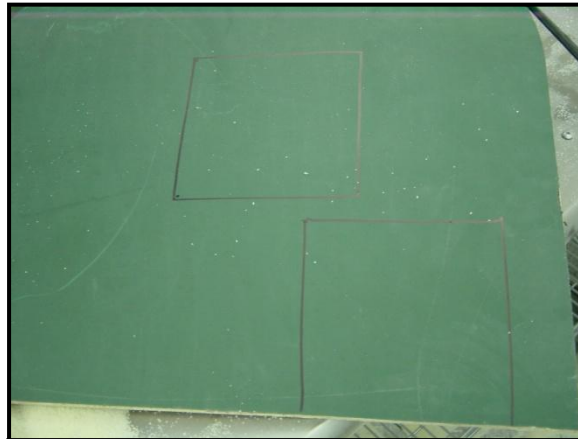
Panel Cut from MC-130 Radome Prior to CHP Blasting
