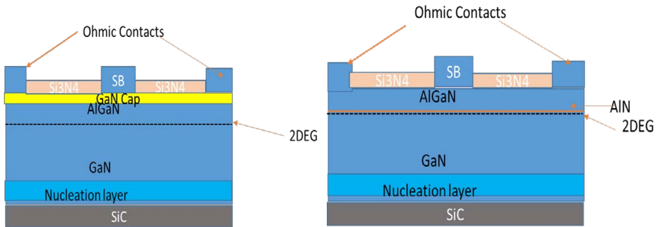
Figure 2.1. The AlGaN/AlN/GaN (left) and the GaN/AlGaN/GaN (right) device structures used in this research.
