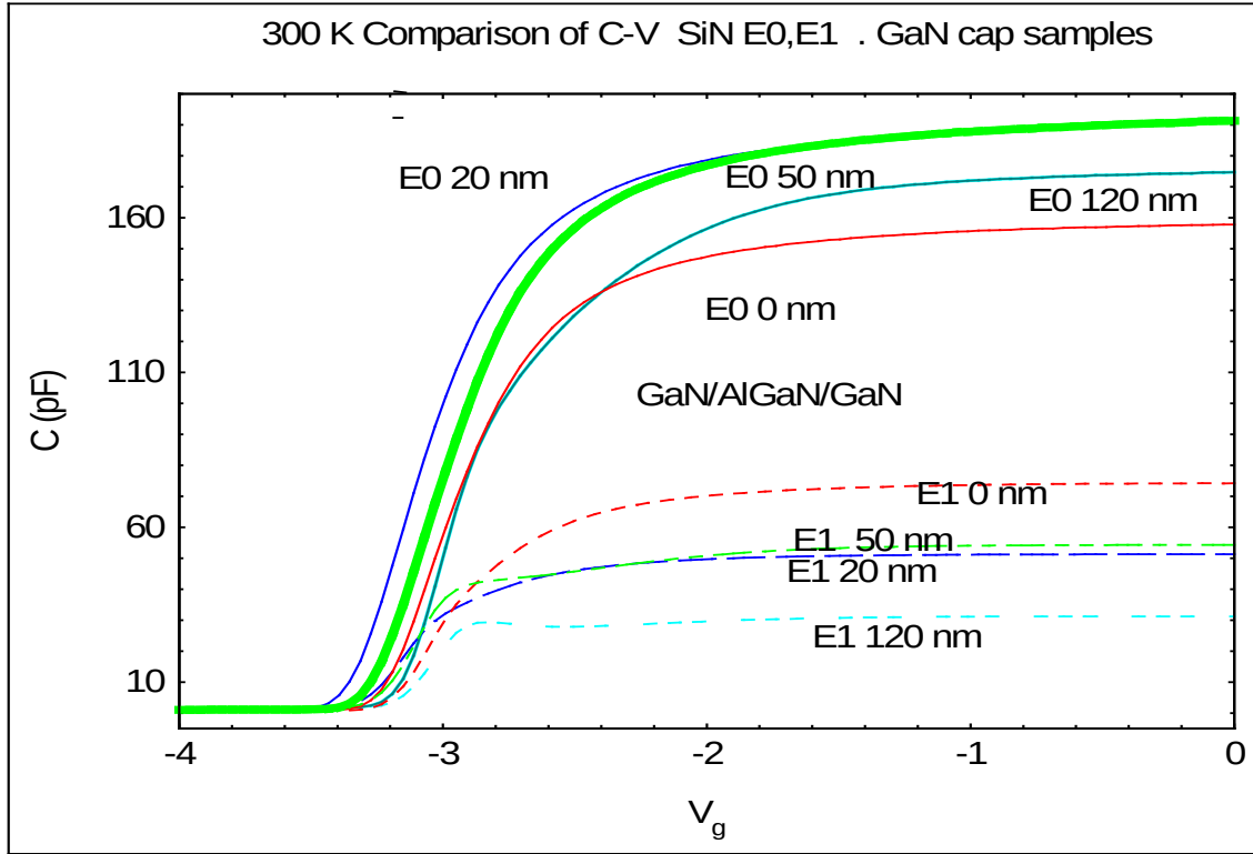
Figure 6.18 300 K comparison of C-V showing effect of variation of \text{Si}_3\text{N}_4 thickness before and after 1 MeV electron irradiation on GaN/AlGaN/GaN.
