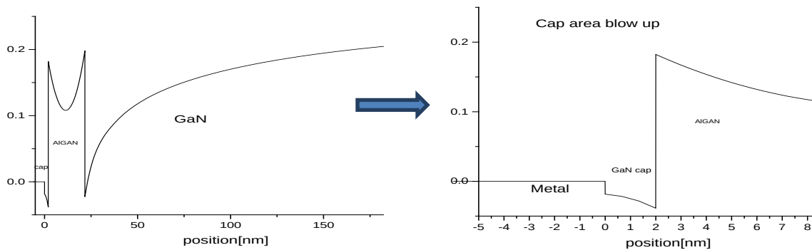
Figure 5.19. Modeled conduction band for GaN (2 nm)/AlGaIn/GaN (left) with enlarged view of the cap area.
