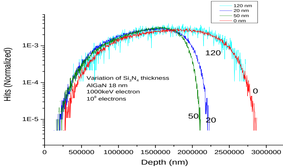
Figure 5.44 Normalized hits by 1 MeV electrons at a fluence of 10^8 \text{ nm}^{-3} as a function of \text{Si}_3\text{N}_4 thickness on AlGaIn (18nm)/AlN (1nm)/GaIn (1700 nm).
