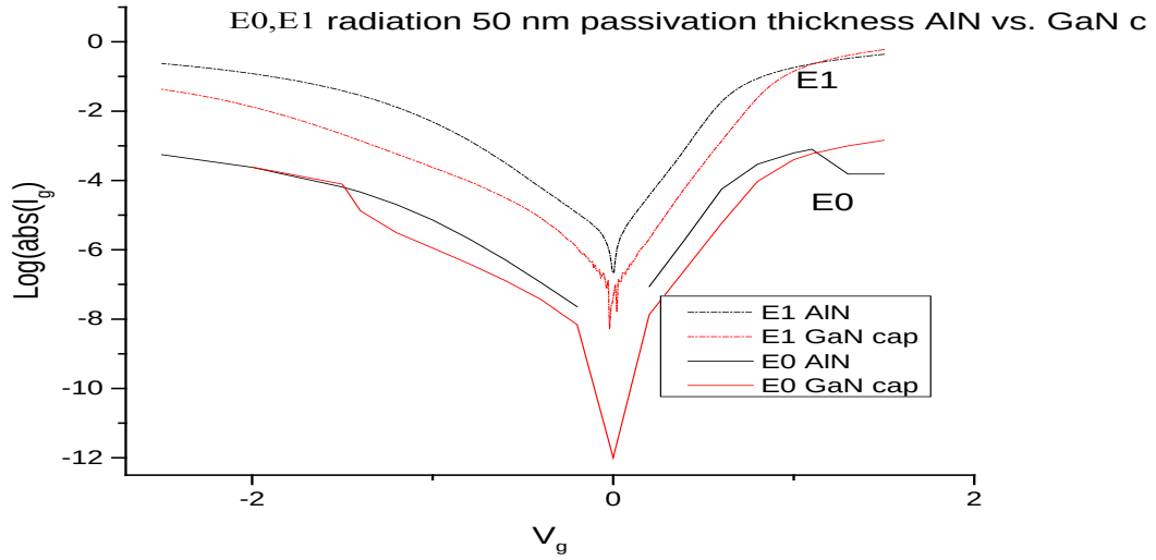
Figure 6.7 The pre (E0) and post(E1) radiation leakage current of both the AlN structure and the GaN cap structure for a 50-nm passivation layer thickness, showing that the GaN cap structure has less leakage.
