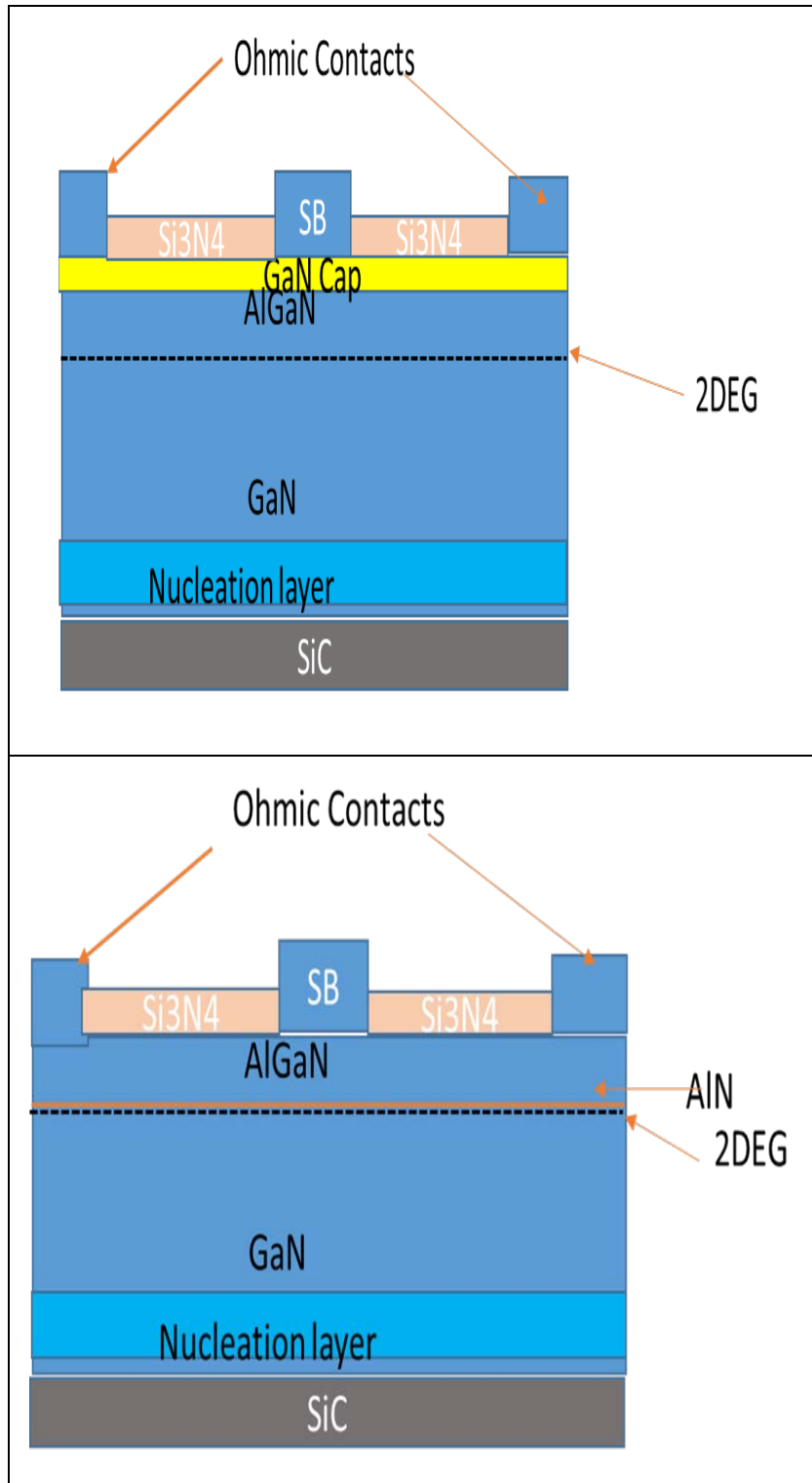
Figure 4.3. Device structures for GaN/AlGaIn/GaN and AlGaIn/AlN/GaN.
