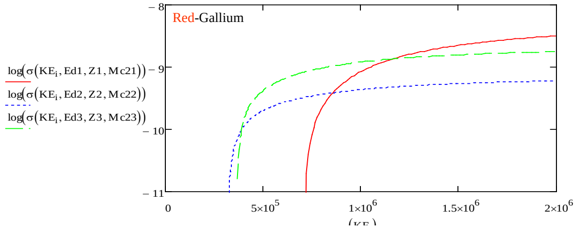
Figure 7.19. Cross section as a function of kinetic energy in AlGaN for Gallium (red), Nitrogen (blue) and Aluminum (green). The log of the cross section times the dose and density will give a defect production rate. Acceptors will be Gallium vacancies, while the nitrogen defects can be donors or acceptors.
