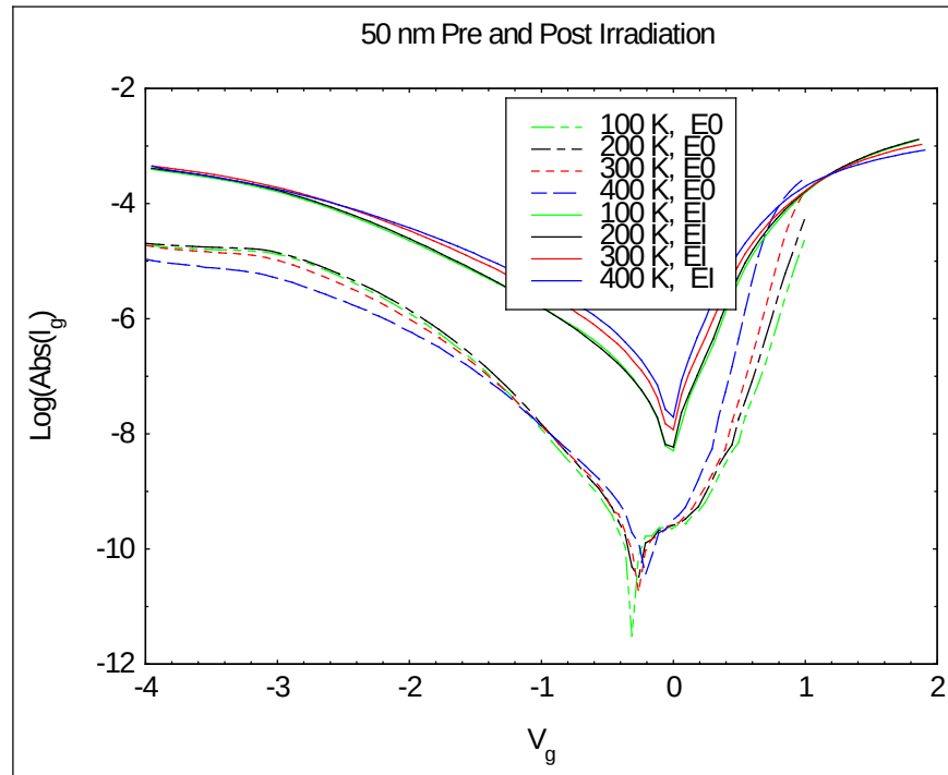
Figure 6.5. Temperature dependence of I_g - V_g after 1-MeV electron irradiation for unpassivated GaN/AlGaIn/GaN.
