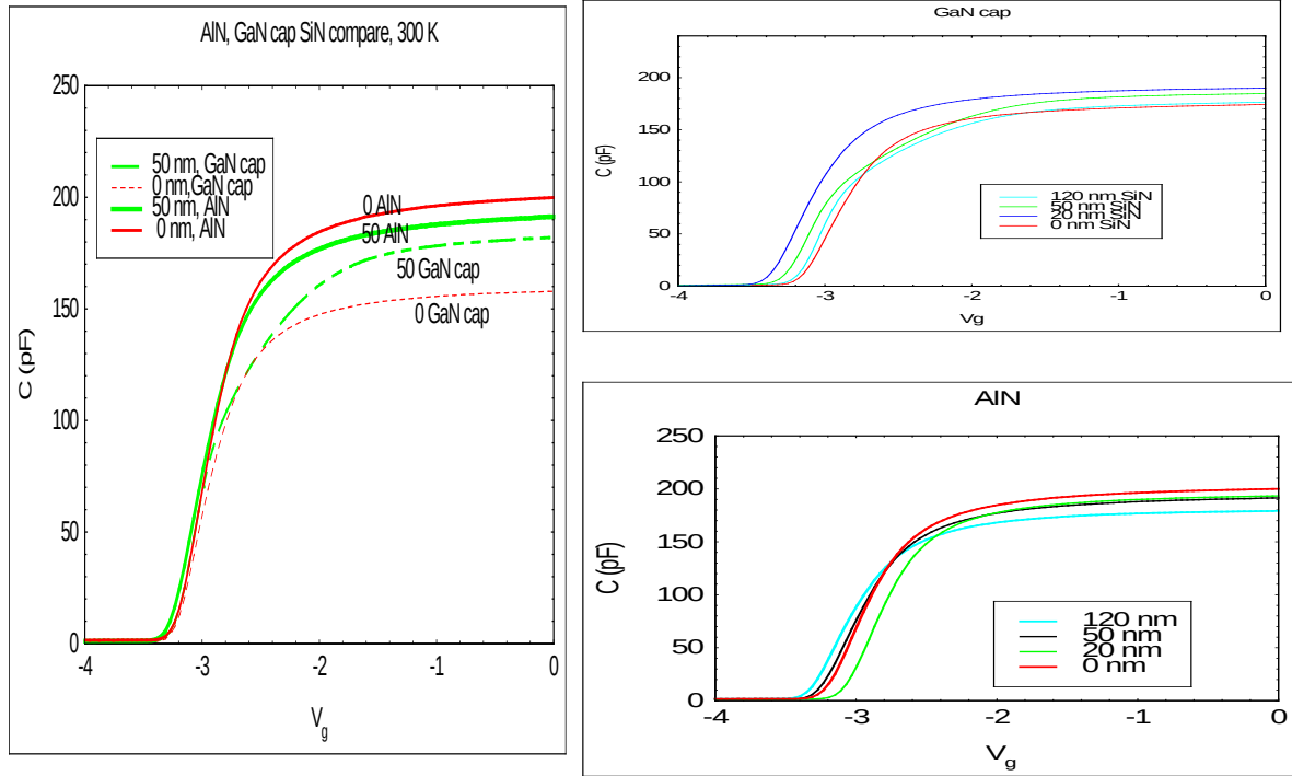
Figure 6.12. Comparison of \text{Si}_3\text{N}_4/\text{AlGaN}/\text{AlN}/\text{GaN} (IQ 15) with \text{Si}_3\text{N}_4/\text{GaN}/\text{AlGaN}/\text{GaN} (IQ 13) room temperature C_g - V_g (left). The unpassivated AlN structure has a higher saturation capacitance, but the opposite is true for the GaN cap structure.
