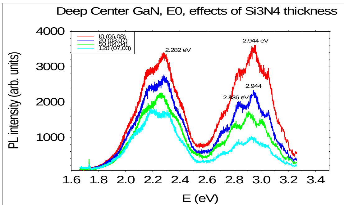
Figure 5.32. E0 Deep center PL with variation of Si 3 N 4 thickness, showing the YL peak at 2.3 eV and the BL peak at 3.0 eV.
