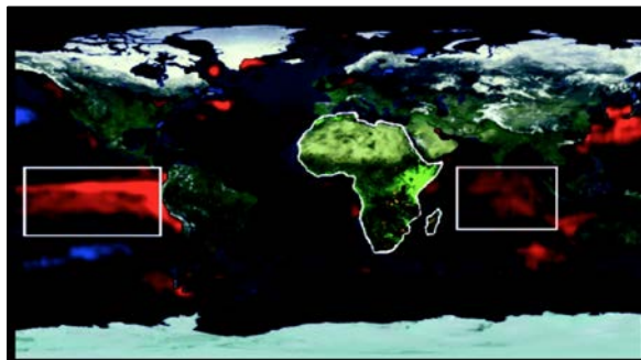
Figure 5. This February 1998 image illustrates the close relationship between ocean temperature (warmer-than-normal ocean temperatures are shown in red, cooler-than-normal temperatures in blue), rainfall, and their impacts on land vegetation (greener-than-normal vegetation shown in light green).
