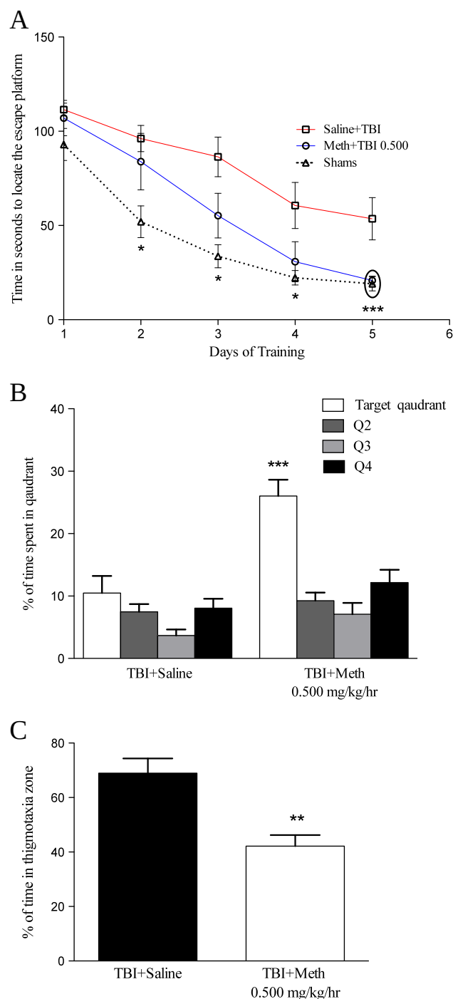
Fig. 4. Treatment with low dose methamphetamine improved learning and memory when delivered 12 h after a severe TBI. (A) Shows latency times over 5 training days for rats treated with saline (red line), or 0.500 mg/kg/h (blue line) beginning 12 h after severe TBI. The dotted black line indicates the latency times for uninjured control rats. (B) Shows the percent time rats spent in each quadrant of the maze searching for the escape platform. The target quadrant (white bars) is where the escape platform had previously been located. Non-target quadrants were Q2–4. (C) Shows the percent of time rats from each treatment group spent within the thigmotaxia zone. n = 8 animals per group. * = p < 0.05 , ** = p < 0.01 , *** = p < 0.001 relative to saline treated controls.
