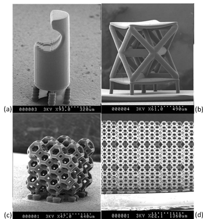
FIG. 8. Complex three-dimensional structures manufactured with the P\mu\text{SL} system. (a) Micro-gripper structure with overhanging gripper and pre-defined curvature. (b) Micro-lattice unit cell structure. (c) Porous structure with tetrakaidehedron unit cell architecture. (d) 5 \times 3 \times 3 \text{ mm}^3 porous structure assembled from multiple porous unit cells from (c) using the step-and-repeat process.
