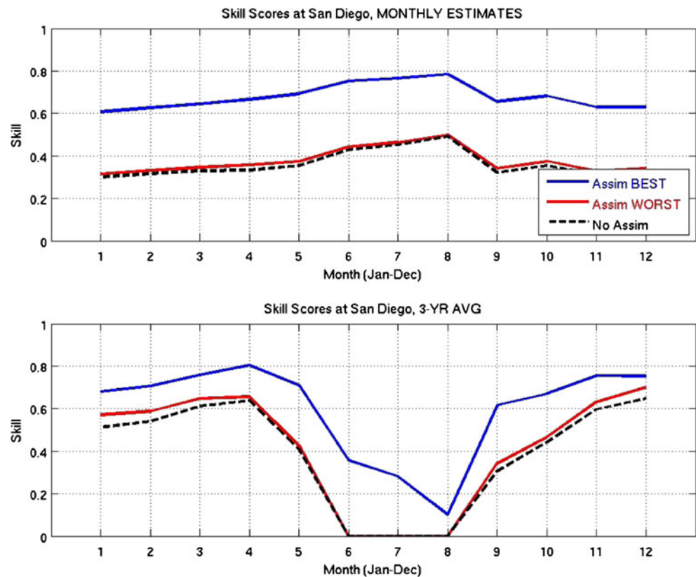
Fig. 12 Skill scores at San Diego site, plotted versus month of the year. Same format as Fig. 8
