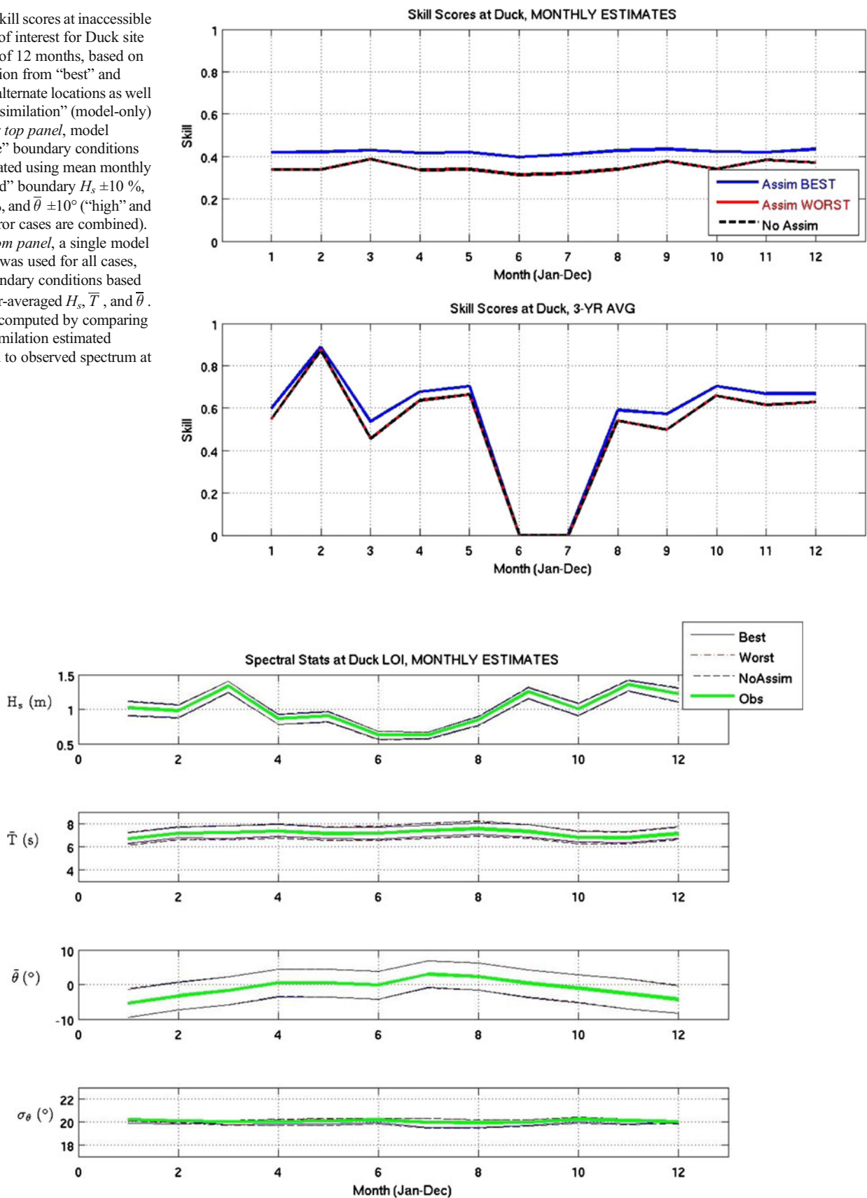
Fig. 9 Spectral statistics at Duck LOI based on monthly estimates, plotted versus month of year. Solid green line is observed values while others represent estimates based on best, worst, and non-assimilation cases for both low and high waves
