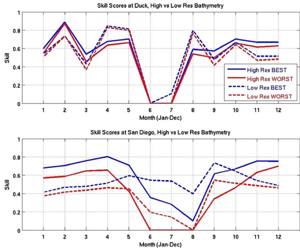
Fig. 18 Spectral skill values at Duck ( top ) and San Diego ( bottom ), including assimilations from “best” (blue) and “worst” (red) alternate locations for high-resolution (solid) and low-resolution (dashed) bathymetry. Model estimates are initialized with 3-year-averaged conditions for 2010–2012
