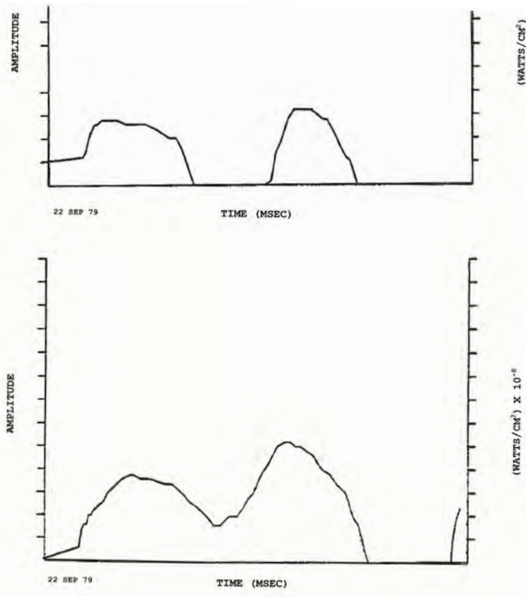
Figure 13-3. Bhangmeter Light Patterns for Event Detected by a Vela Satellite on September 22, 1979.
