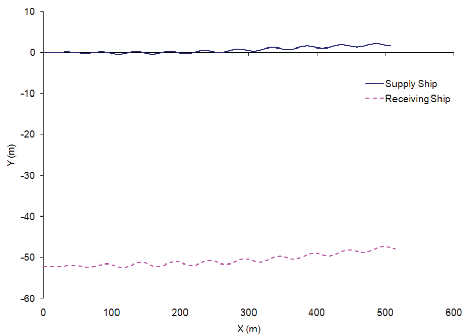
Figure 58: Ship trajectories during the first 80 s – Test Case 9.
