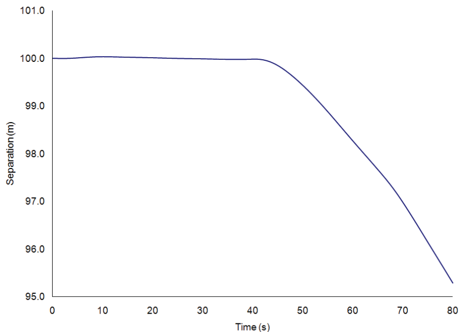
Figure 29: Change in distance between ships during the first 80 s – Test Case 2.
