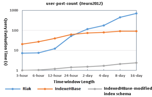
Fig. 21. Query evaluation time comparison with modified meme index table schema
