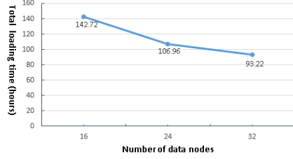
Fig. 13. Historical data loading scalability to cluster size
