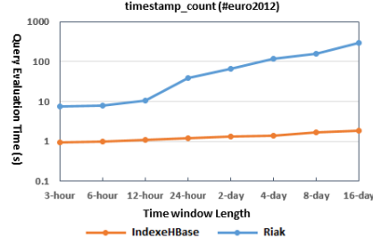
Fig. 18. Query evaluation time for “timestamp-count”
