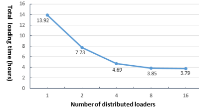
Fig. 14. Results for streaming data loading test
