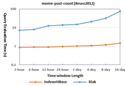
Fig. 17. Query evaluation time for “meme-post-count”
