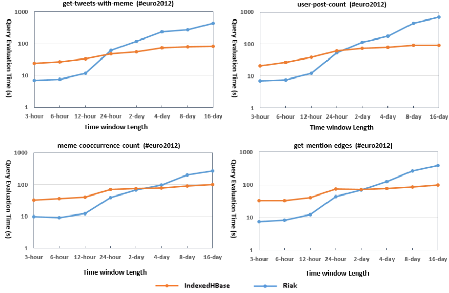
Fig. 19. Query evaluation time for queries requiring MapReduce on both platforms
