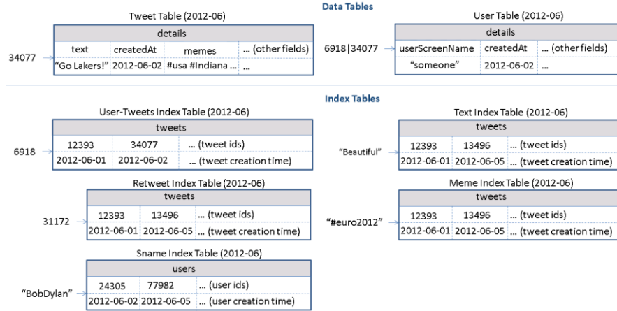
Fig. 5. Table schemas used in IndexedHBase for Truthy
