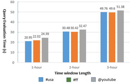
Fig. 15. Query evaluation time with separate meme and time indices (Riak)
