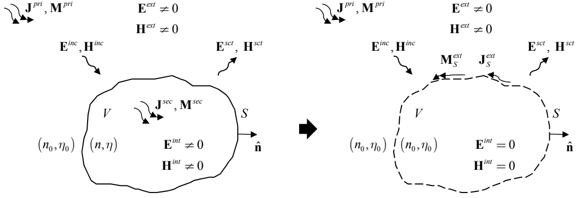
Figure 3. The exterior problem associated with using surface equivalence. Here, the interior region contains null fields; thus, equivalent sources in the form of surface current densities radiate the scattered fields. These equivalent sources radiate in the presence of the primary source and incident fields. Superposition of the incident and scattered fields replicate the exterior fields which propagate throughout free space.
