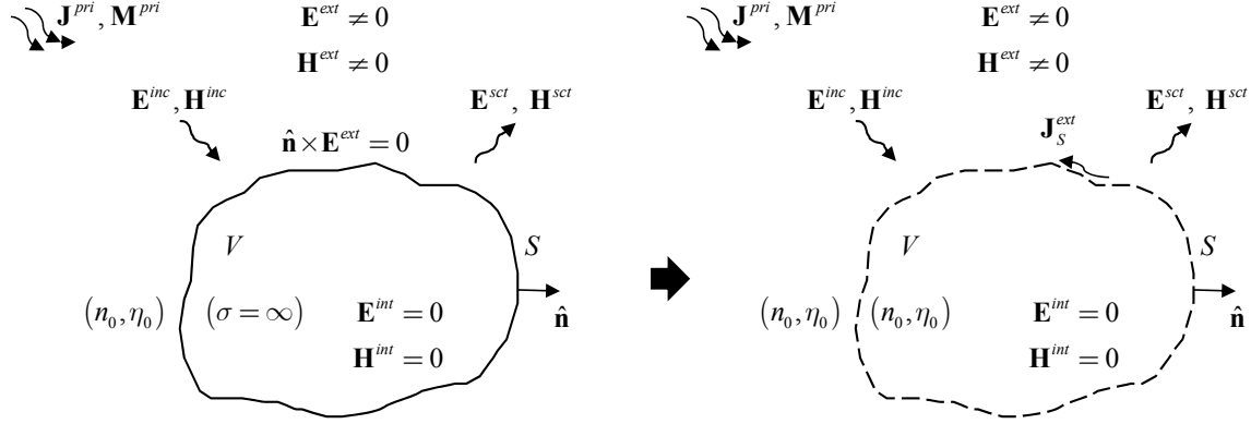
Figure 4. The interior region within a perfect electrical conductor contains null fields. As such, only an exterior problem exists when using surface equivalence. The resulting electric current density radiates the scattered fields and superposition with the known incident fields replicates the exterior fields which propagate throughout free space.
