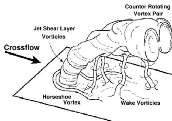
Figure 4. Schematic of various vortex structures in JICF, After Fric & Roshko [3]
