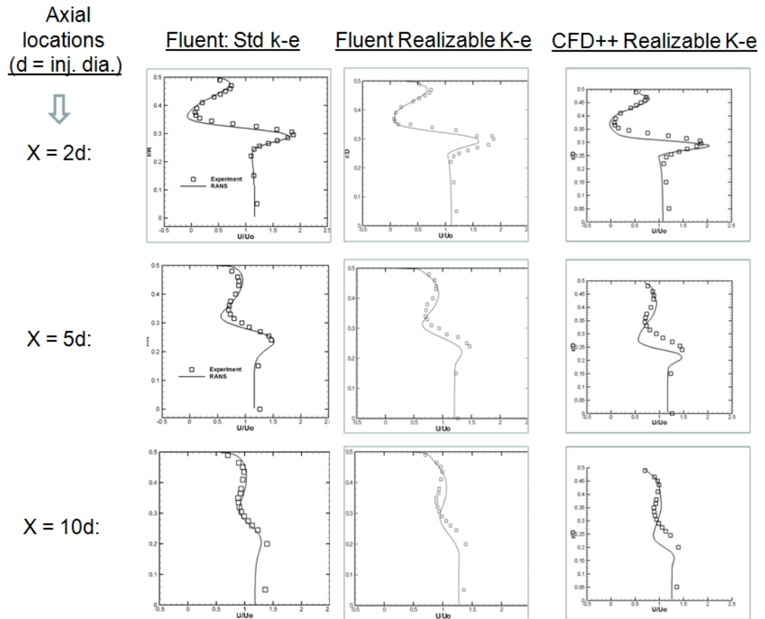
Figure 8. Experimental data vs. predicted radial profiles of the axial velocity using standard k- \epsilon and realizable k- \epsilon
