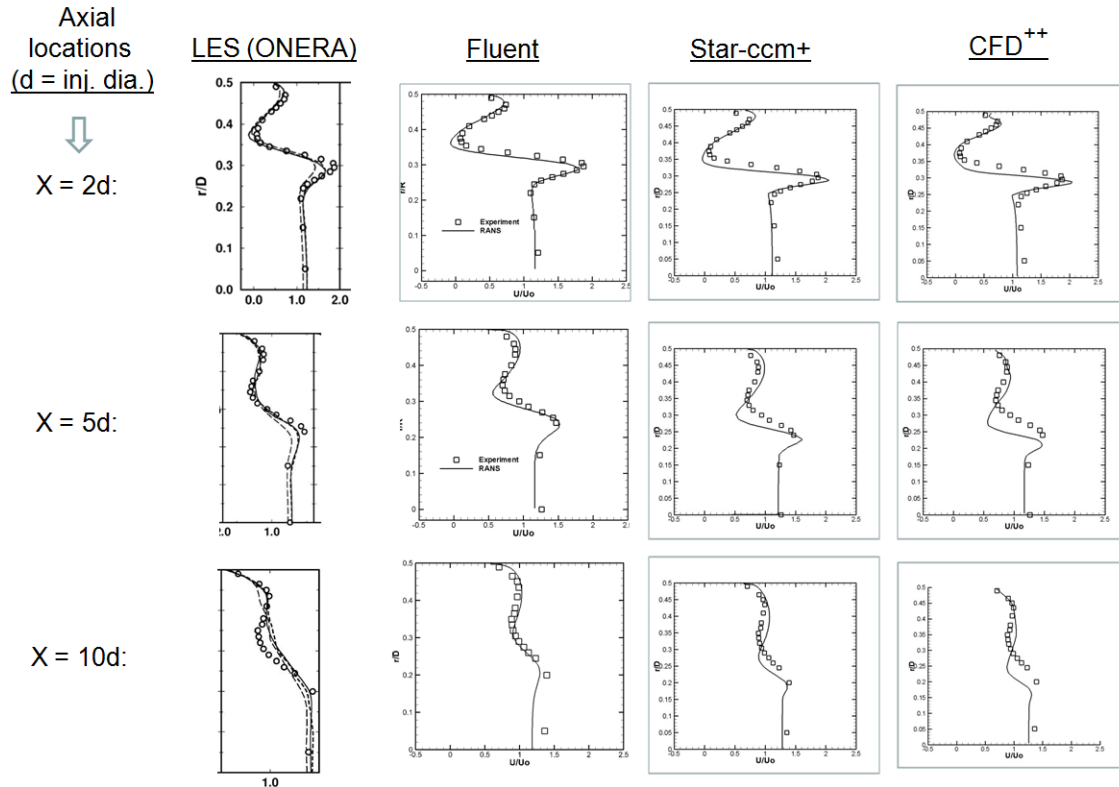
Figure 7. Predicted vs. experimental radial profiles of the axial velocity at different axial locations
