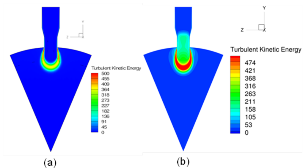
Figure 9. Predicted turbulent kinetic energy with Fluent (a) Standard k- \epsilon with standard wall function, (b) realizable k- \epsilon with enhanced wall treatment
