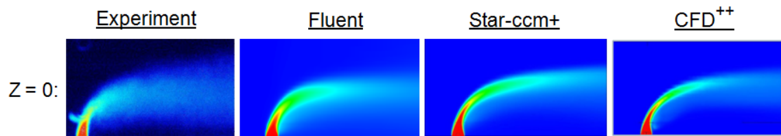
Figure 8. Jet mass fraction distribution
