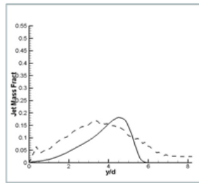
Figure 9. Computational and experimental jet concentration profiles at x = 2d, 5d, and 10d
