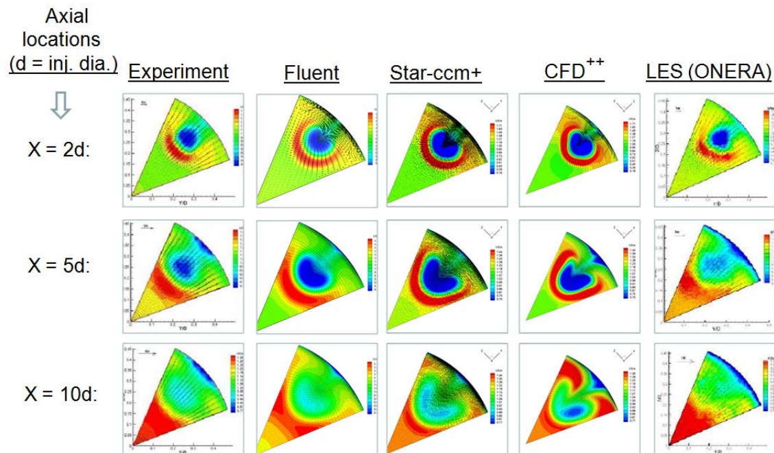
Figure 6. Axial velocity distribution at different axial stations
