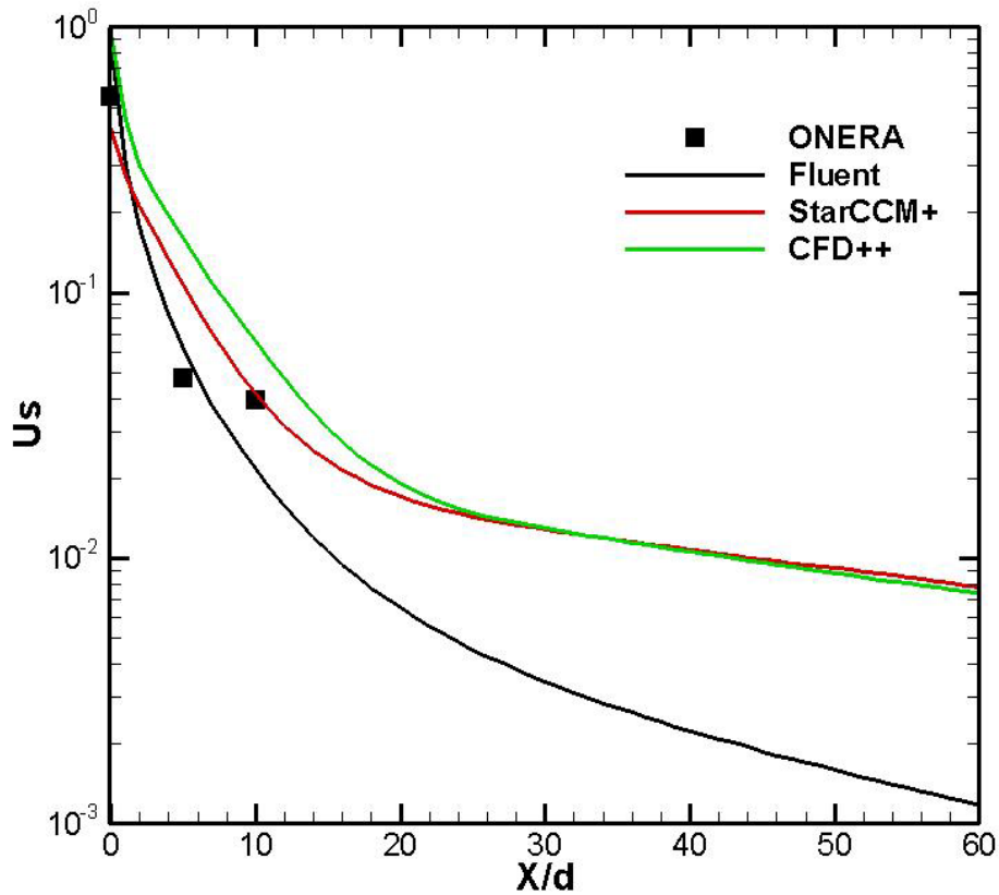
Figure 10. Experimental and predicted unmixedness
