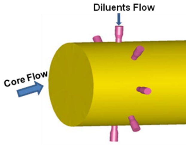
Figure 1. Geometry in the vicinity of the jet injection system.
